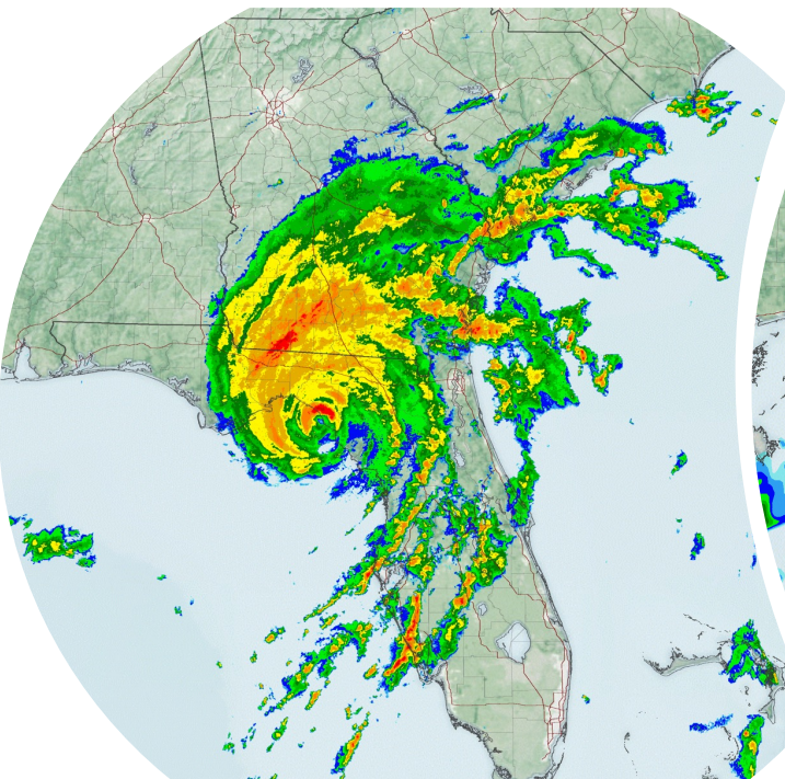
US Observed Radar 941 hPa : 115 Kt
