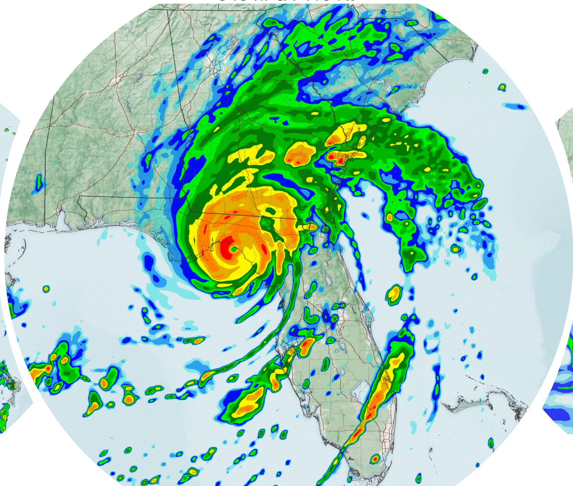
Simulated Radar [dBZ]
