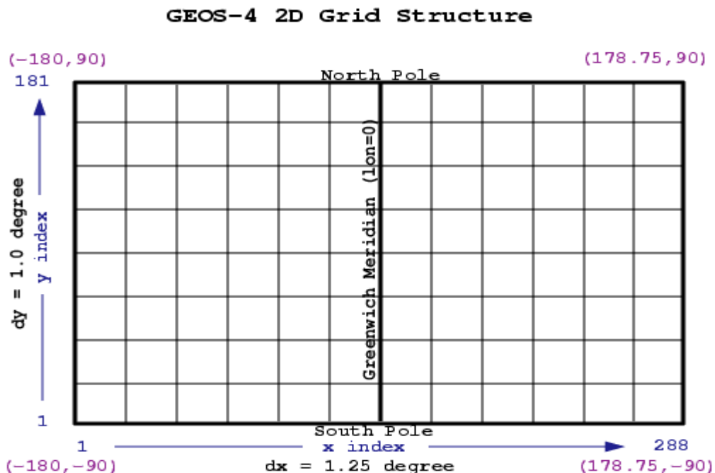
Figure 4-1: 1.25 x 1.0 degree horizontal grid. The origin is at lower-left corner (-180W, -90S). \text{lon} = -180 + (x-1) * dx \text{lat} = -90 + (y-1) * dy
