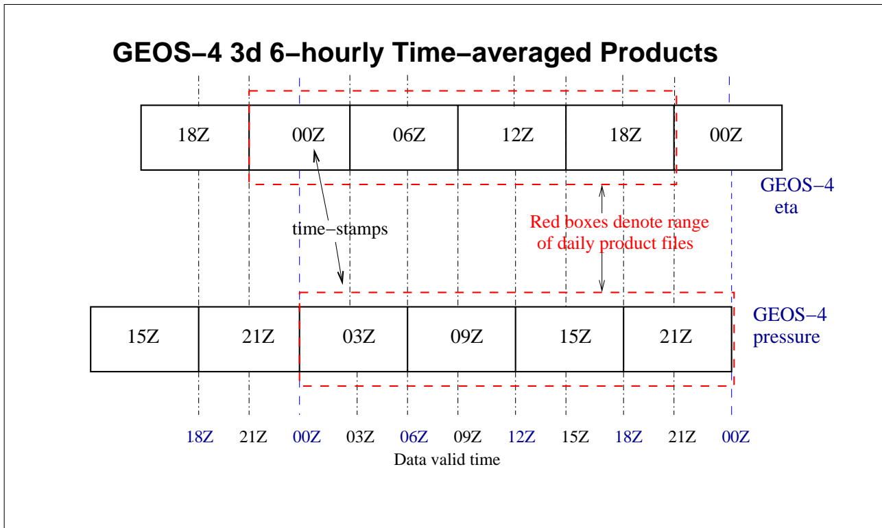
Figure 1 - This is a graphical representation of the averaging periods for GEOS-4 3D time-averaged products. Note that eta-layer products are centered on synoptic times while pressure-level products span the range between synoptic times.
