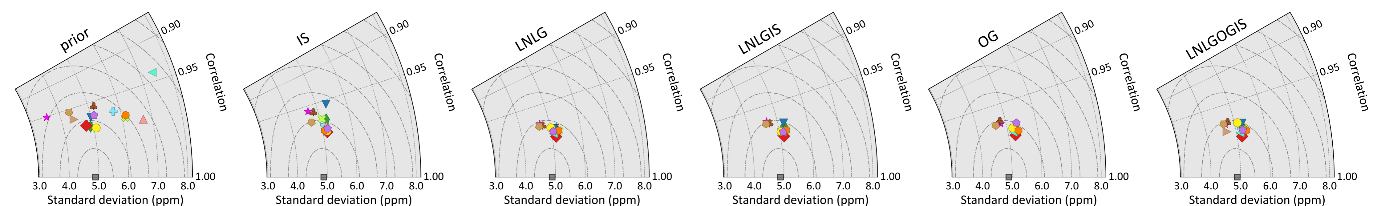
Saga, Kyushu, Japan ■ TCCON + CSU ◆ Ames × COLA ▼ UT ★ CMS-Flux ▲ WOMBAT ♣ JHU ◆ TM5-4DVAR ◀ OU ● CT ▶ Weir ● CAMS ◆ Baker ● NIES
