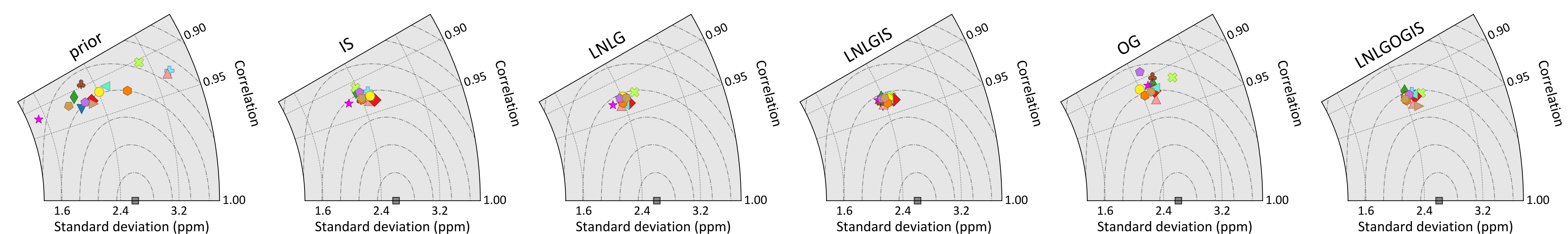
JPL, California, USA ■ TCCON + CSU ◆ Ames ✕ COLA ▼ UT ★ CMS-Flux ▲ WOMBAT ♣ JHU ◆ TM5-4DVAR ◀ OU ● CT ▶ Weir ● CAMS ◆ Baker ● NIES
