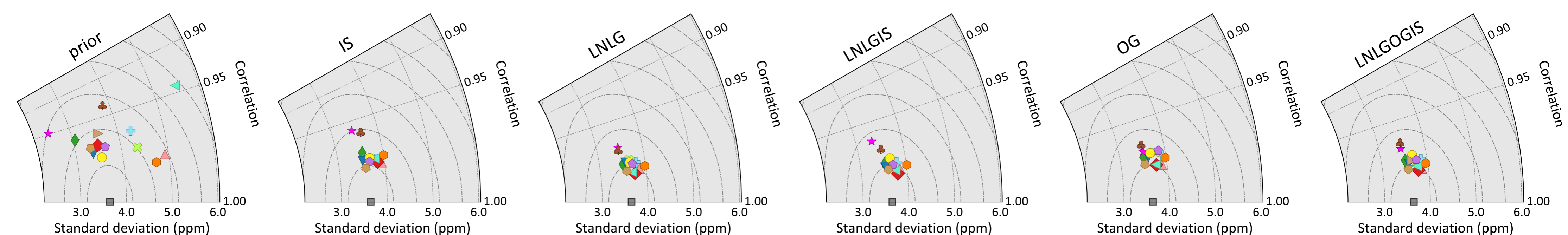
Izaña, Tenerife, Spain ■ TCCON + CSU ◆ Ames × COLA ▼ UT ★ CMS-Flux ▲ WOMBAT ♣ JHU ◆ TM5-4DVAR ◀ OU ● CT ▶ Weir ● CAMS ◆ Baker ● NIES
