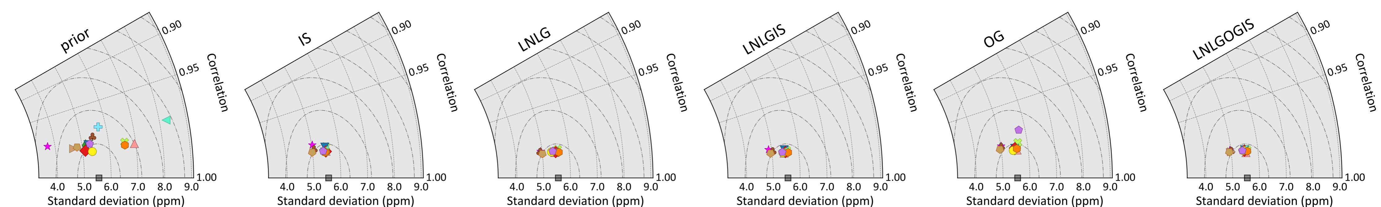
Edwards, California, USA ■ TCCON ■ CSU ◆ Ames ✕ COLA ▼ UT ★ CMS-Flux ▲ WOMBAT ♣ JHU ◆ TM5-4DVAR ▲ OU ● CT ▶ Weir ● CAMS ◆ Baker ▶ NIES
