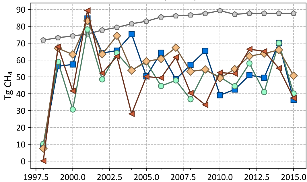
Asia (Fossil)
