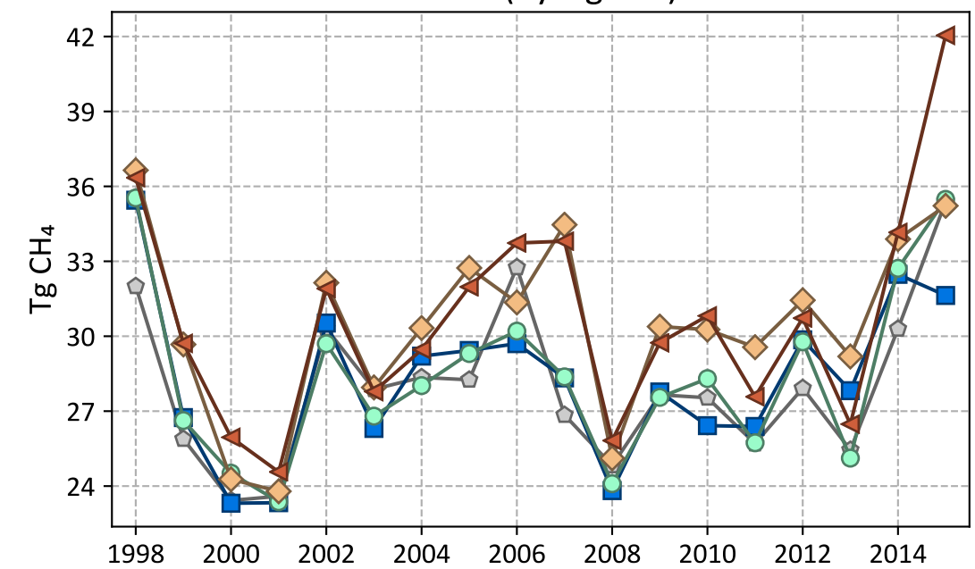
Globe (Pyrogenic)
