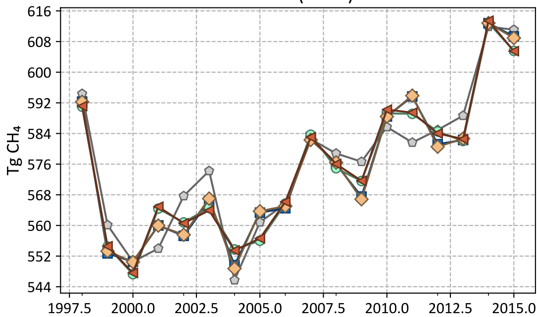
Globe (Fossil)
