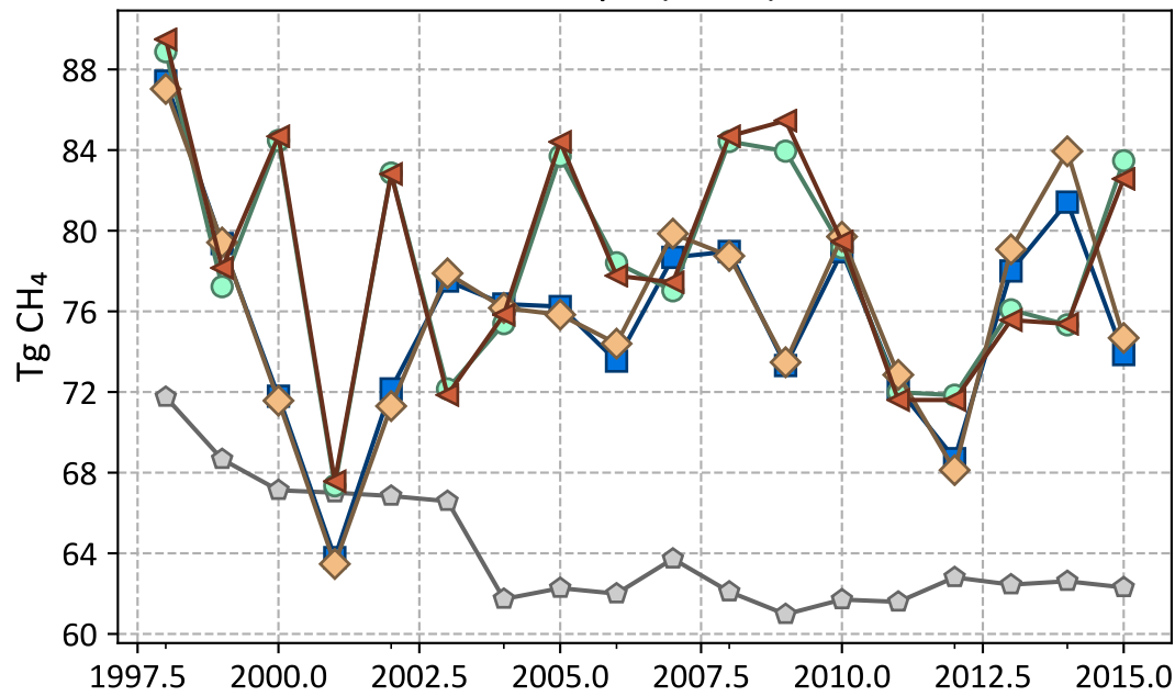
Europe (Fossil)
