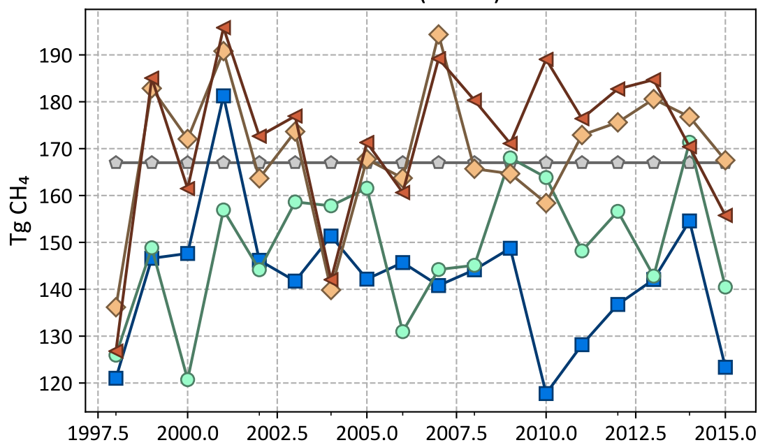
Globe (Fossil)
