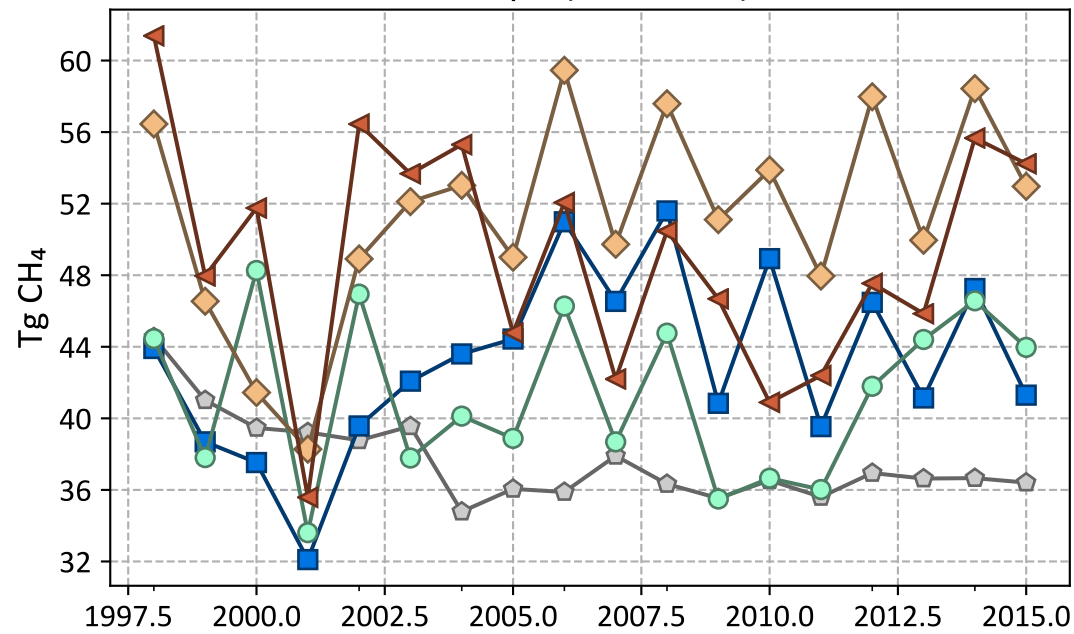
Europe (Pyrogenic)
