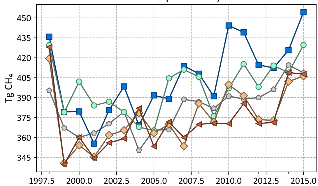
Globe (Pyrogenic)
