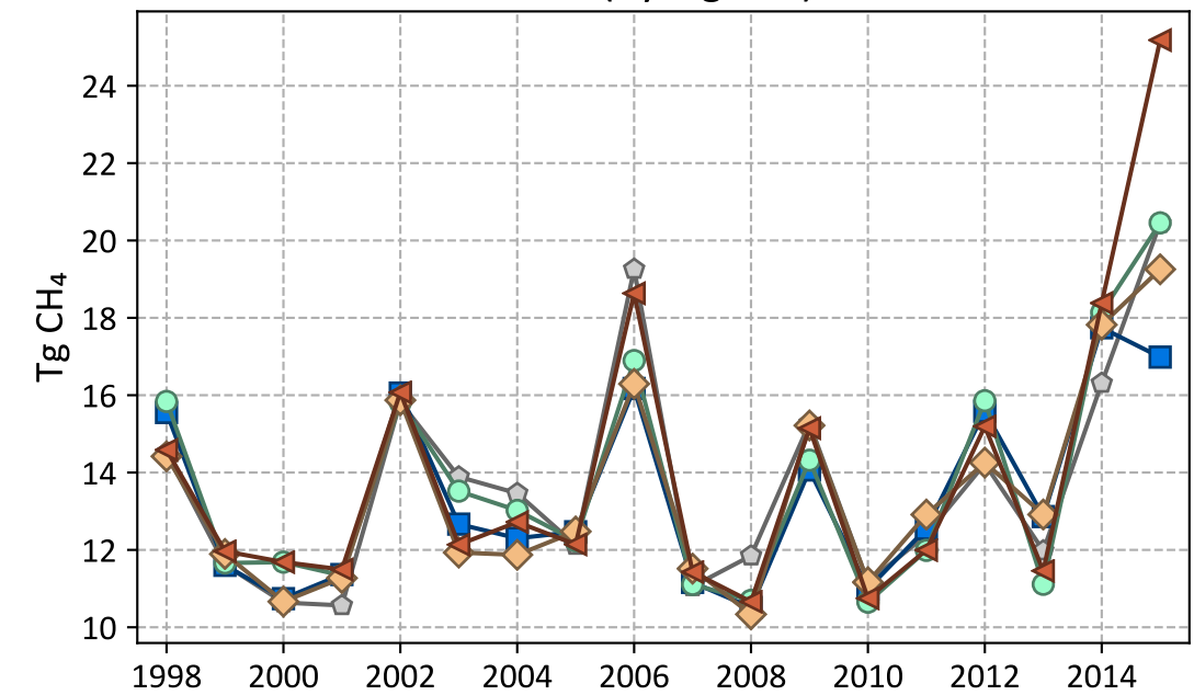
Asia (Pyrogenic)
