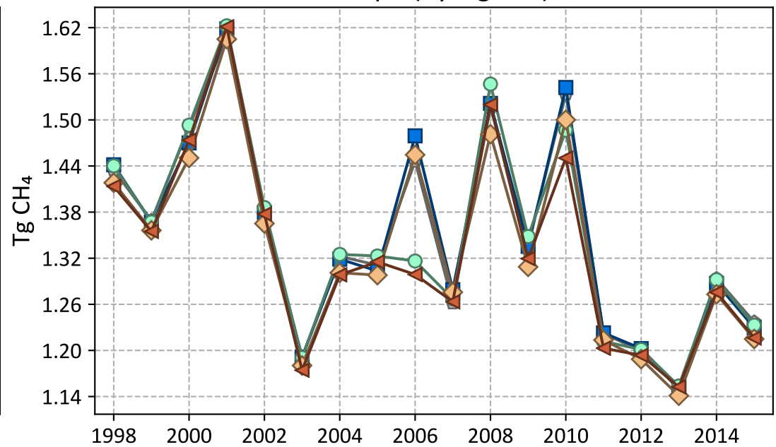
Europe (Pyrogenic)
