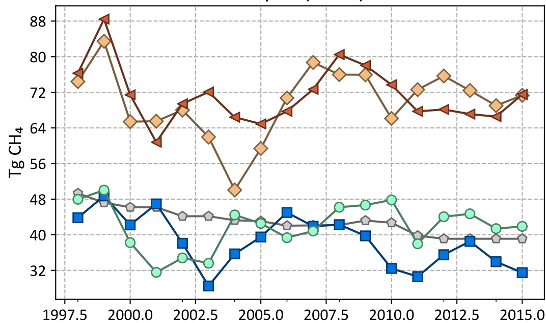
Tropics (Fossil)
