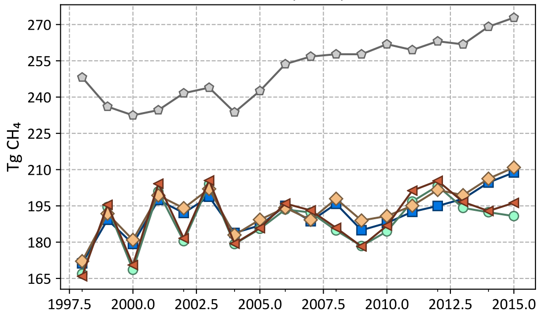
Asia (Fossil)
