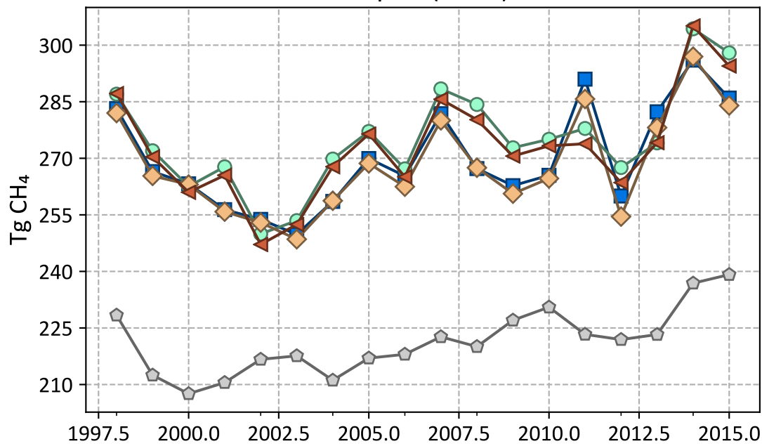
Tropics (Fossil)
