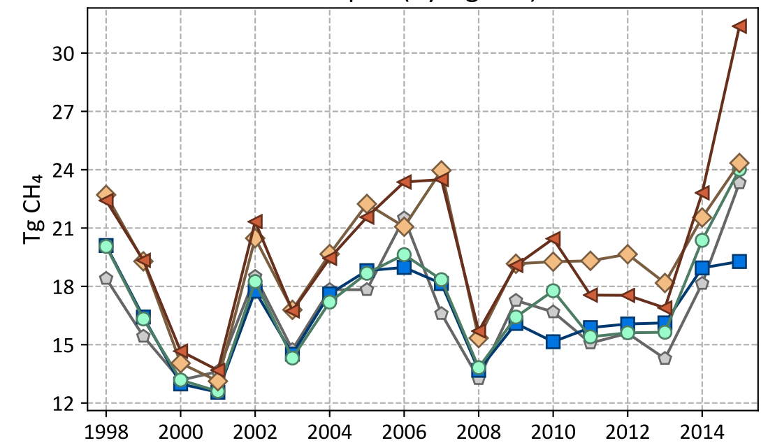
Tropics (Pyrogenic)
