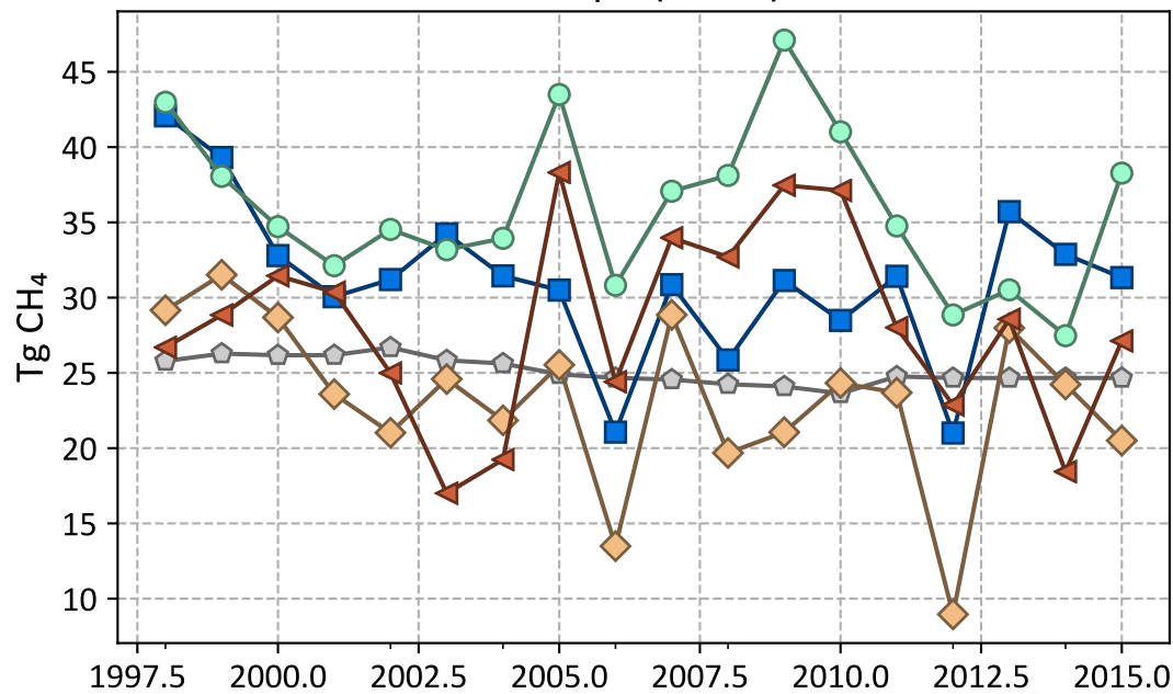
Europe (Fossil)
