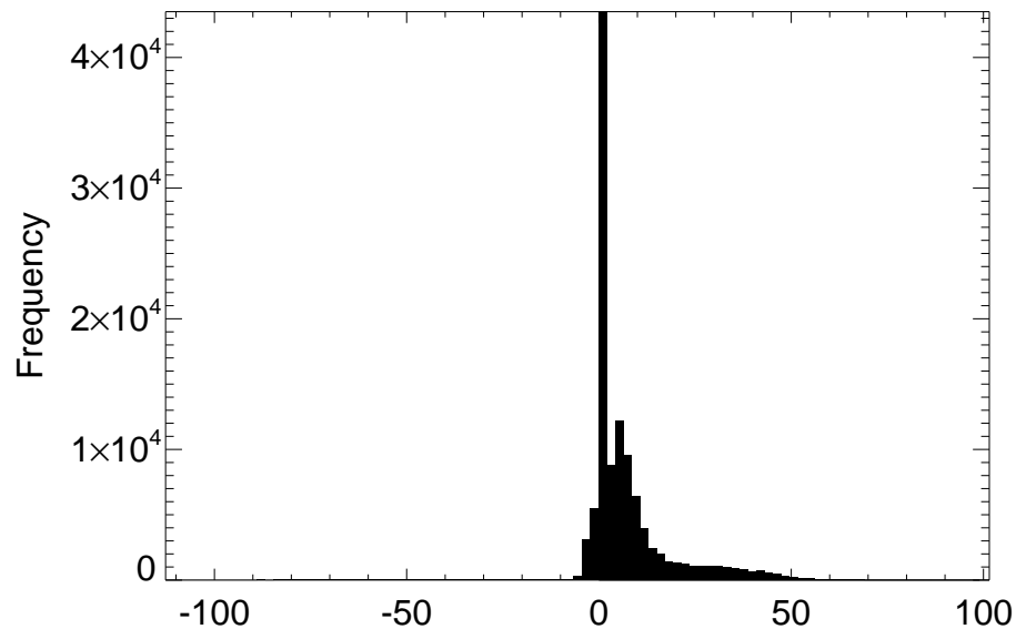
Distribution of SWLAND difference for month 01
