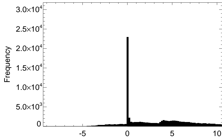
Distribution SWLAND difference for month 03
