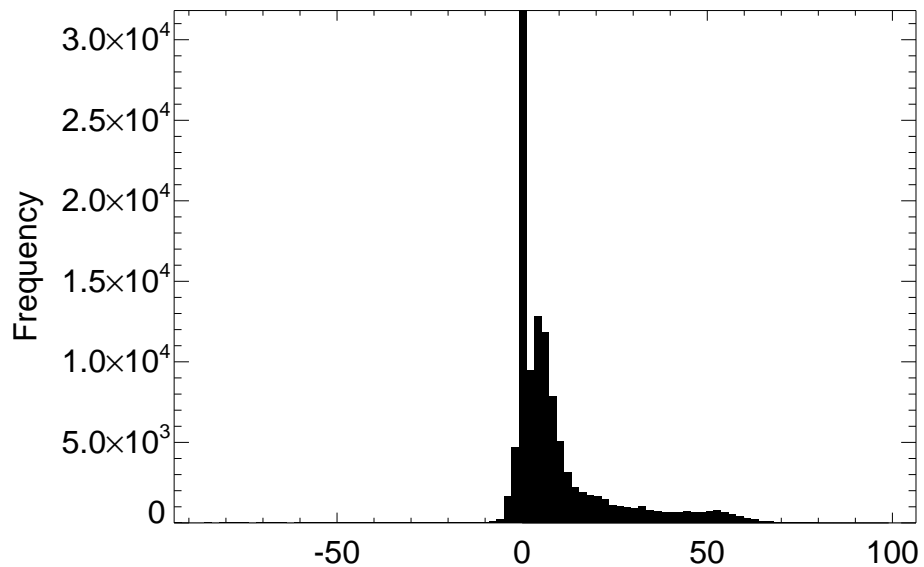
Distribution of SWLAND difference for month 03
