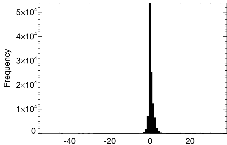
Distribution of LHLAND difference for month 08
