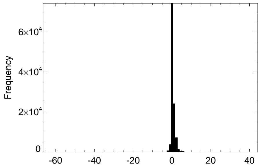
Distribution of LHLAND difference for month 04
