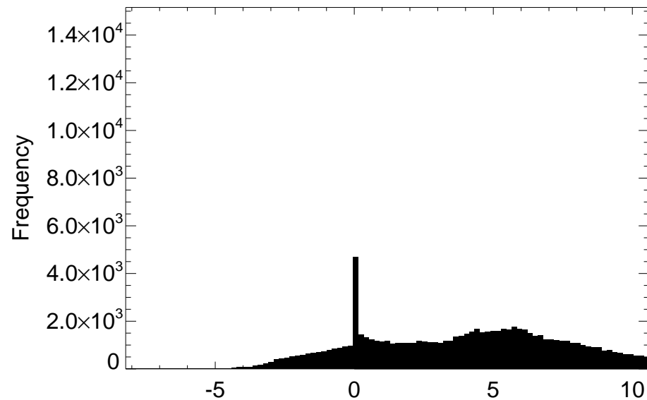
Distribution SWLAND difference for month 05
