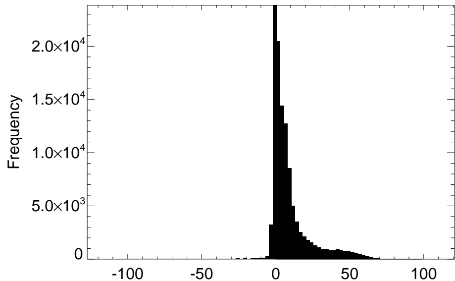
Distribution of SWLAND difference for month 10
