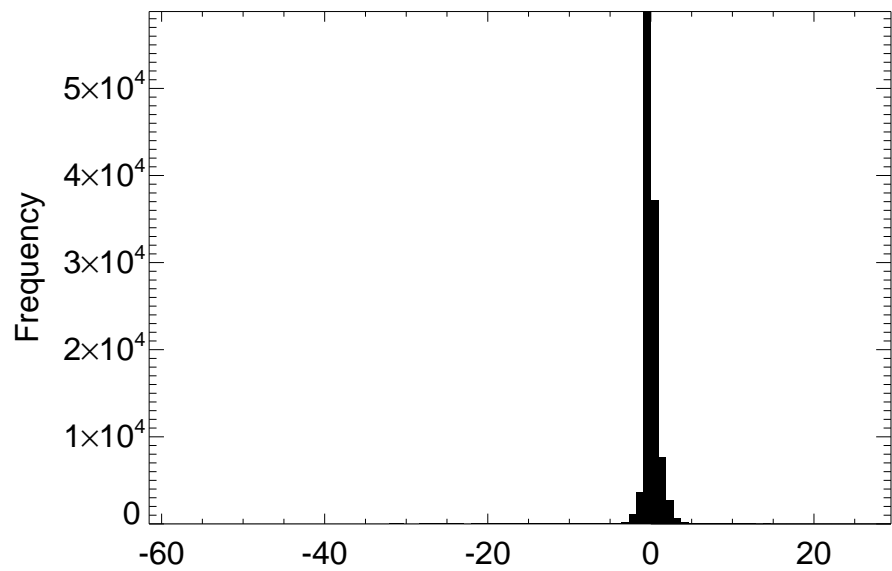
Distribution of LHLAND difference for month 12
