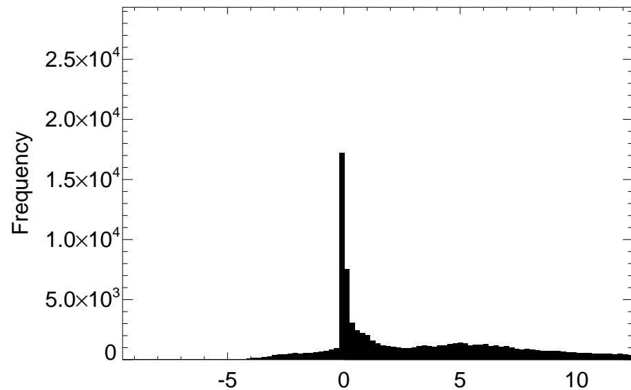
Distribution SWLAND difference for month 11
