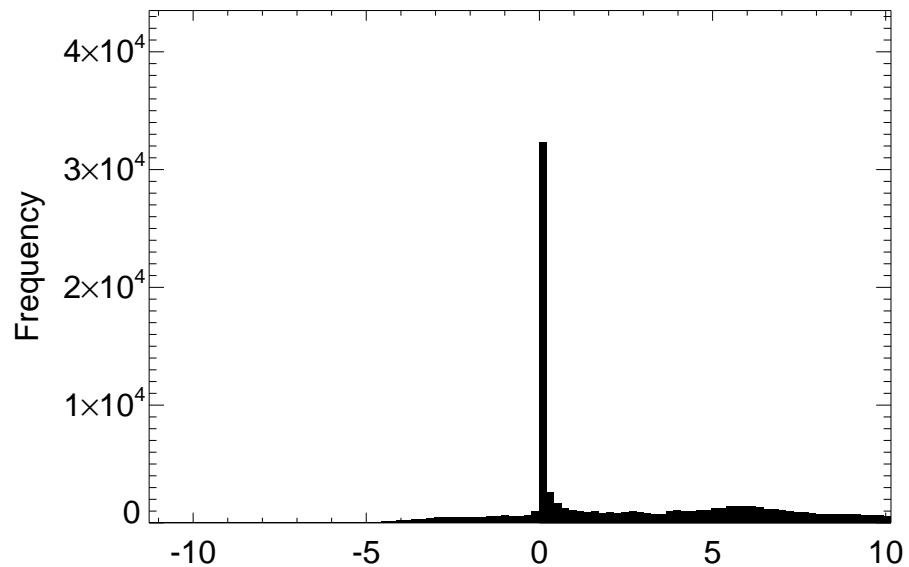
Distribution SWLAND difference for month 01
