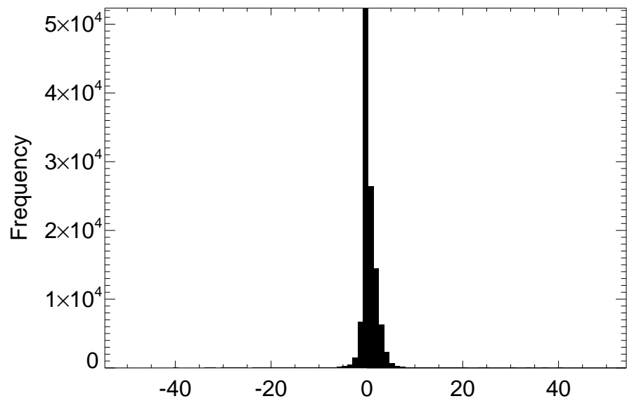
Distribution of LHLAND difference for month 07
