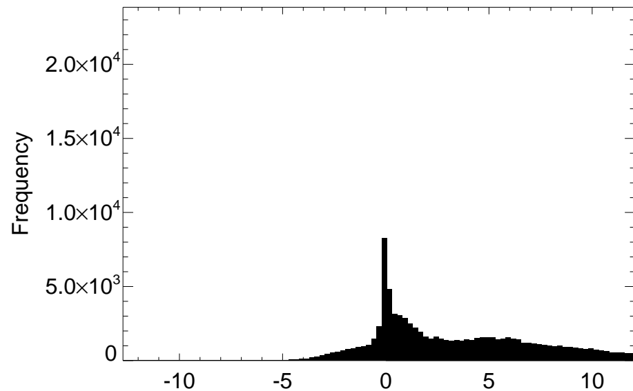
Distribution SWLAND difference for month 10
