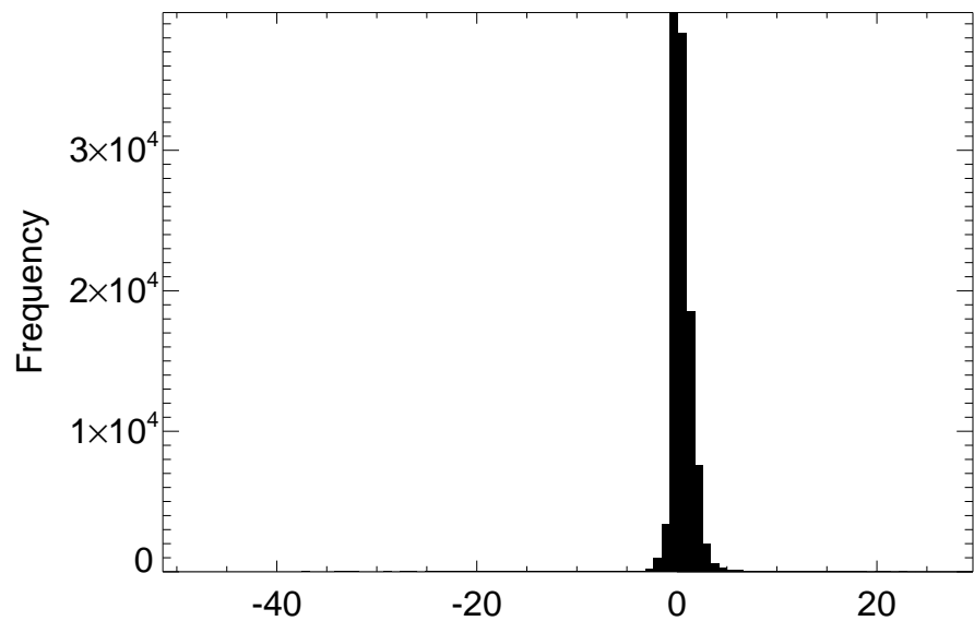
Distribution of LHLAND difference for month 05
