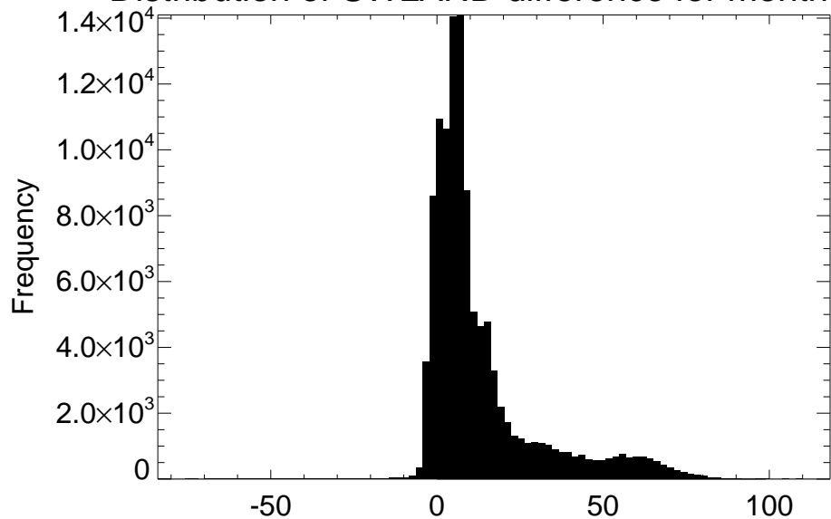
Distribution of SWLAND difference for month 06
