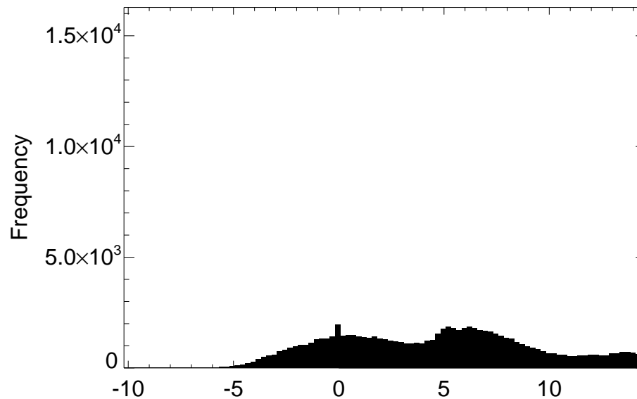
Distribution SWLAND difference for month 07
