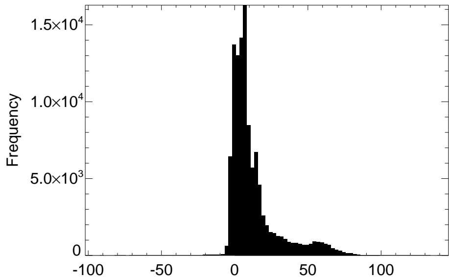
Distribution of SWLAND difference for month 07
