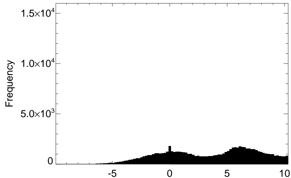
Distribution SWLAND difference for month 08
