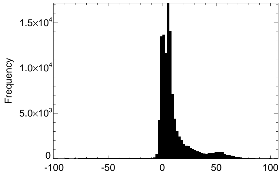
Distribution of SWLAND difference for month 09
