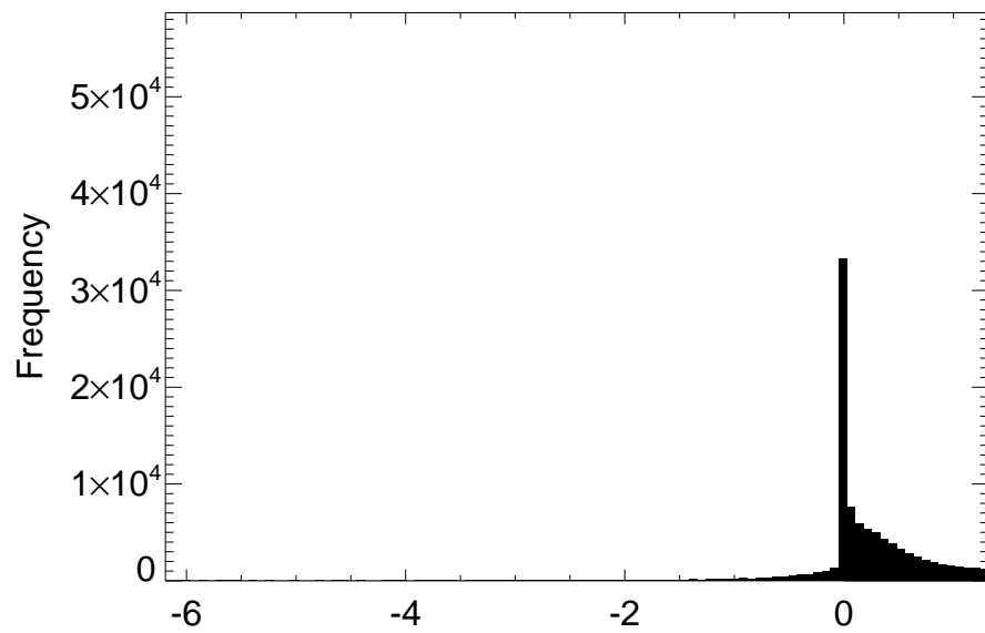
Distribution of LHLAND difference for month 01
