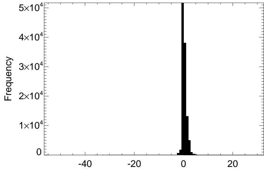
Distribution of LHLAND difference for month 03
