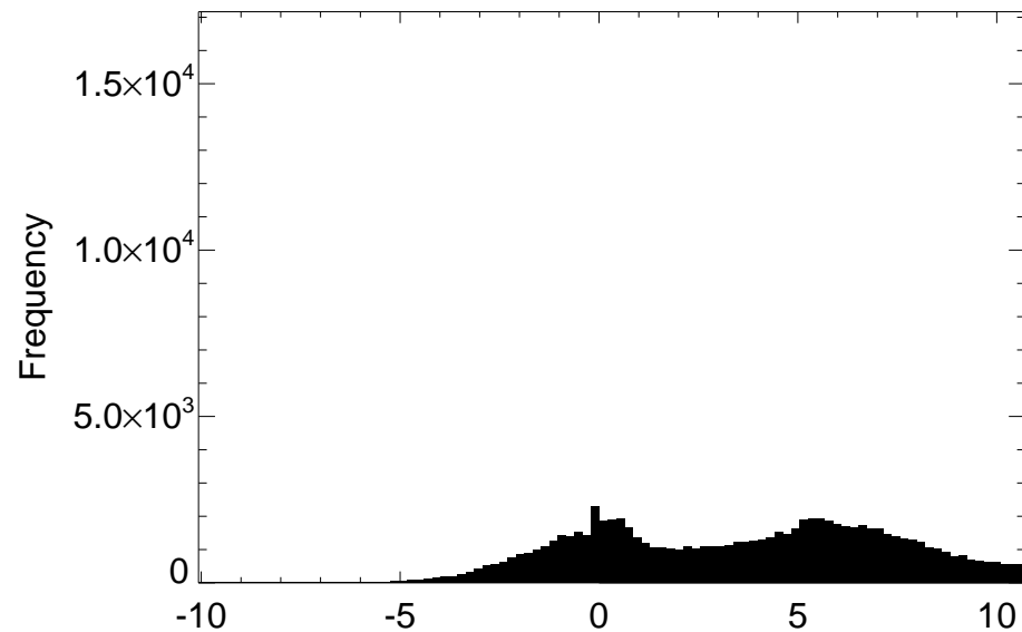
Distribution SWLAND difference for month 09
