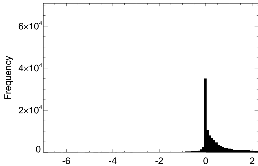
Distribution of LHLAND difference for month 02
