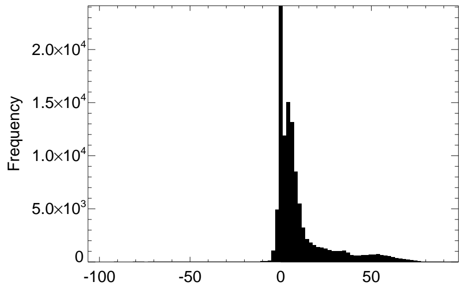
Distribution of SWLAND difference for month 04
