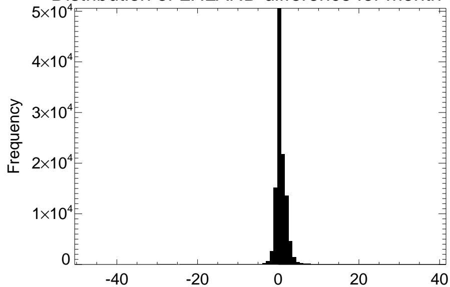
Distribution of LHLAND difference for month 06
