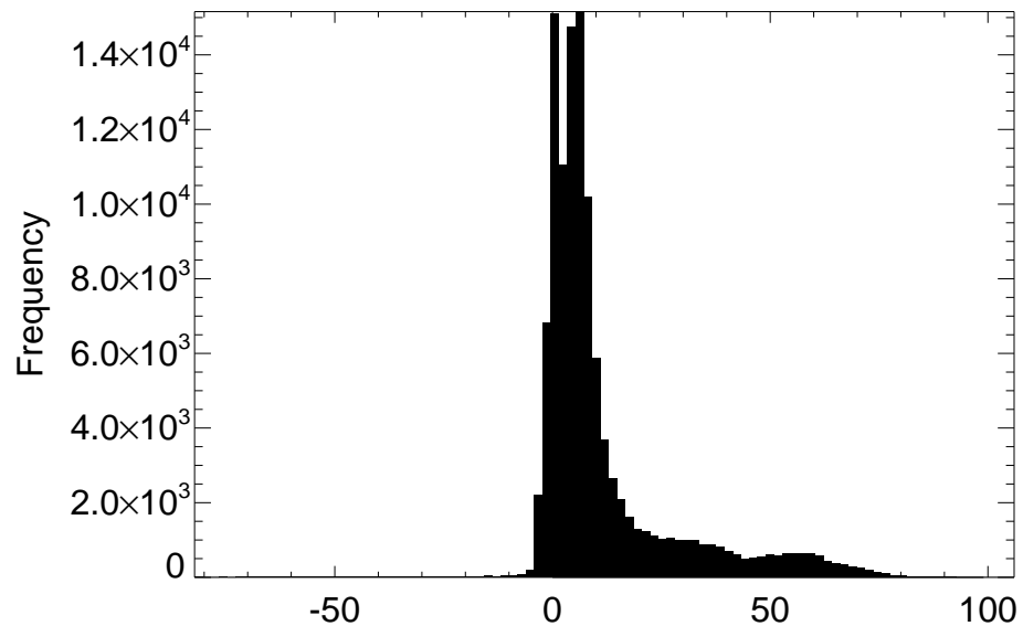
Distribution of SWLAND difference for month 05
