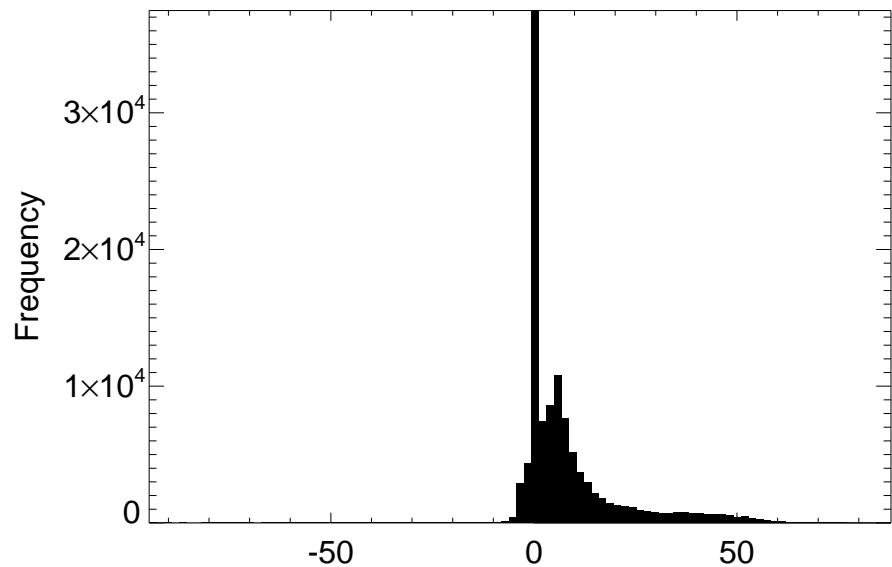
Distribution of SWLAND difference for month 02
