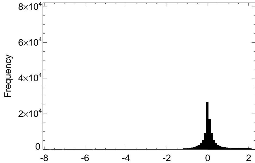
Distribution of LHLAND difference for month 10
