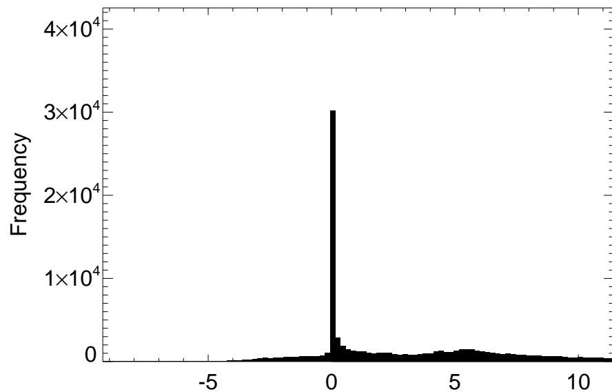
Distribution SWLAND difference for month 12
