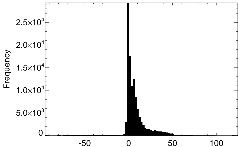
Distribution of SWLAND difference for month 11
