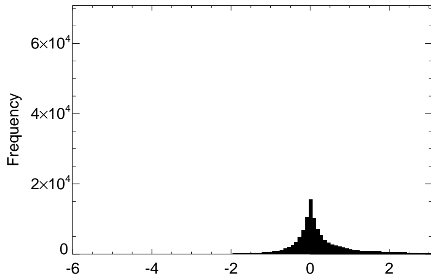
Distribution of LHLAND difference for month 09
