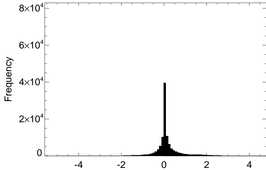
Distribution of LHLAND difference for month 11
