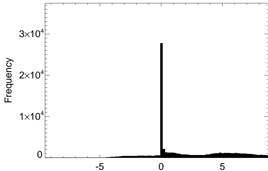
Distribution SWLAND difference for month 02
