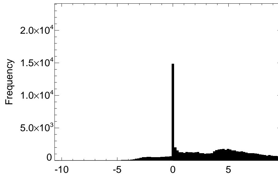
Distribution SWLAND difference for month 04
