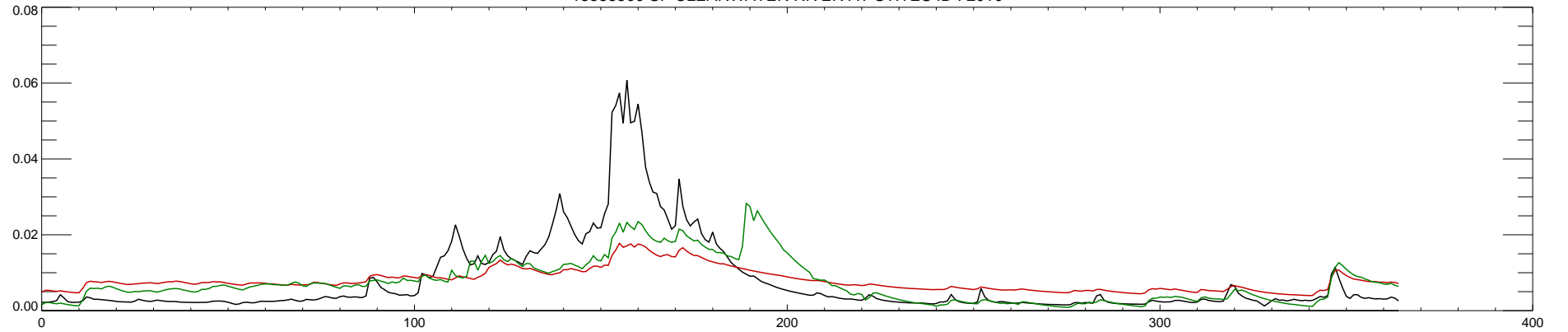
13338500 SF CLEARWATER RIVER AT STITES ID : 2010
