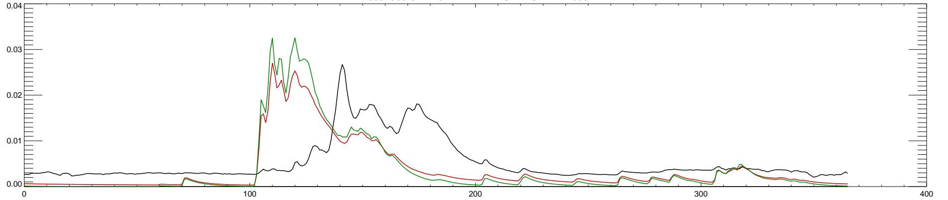
13302500 SALMON RIVER AT SALMON ID : 2009
