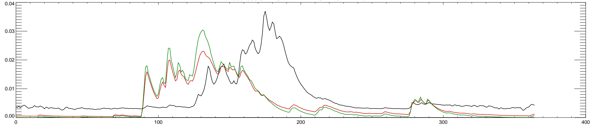
13302500 SALMON RIVER AT SALMON ID : 2012
