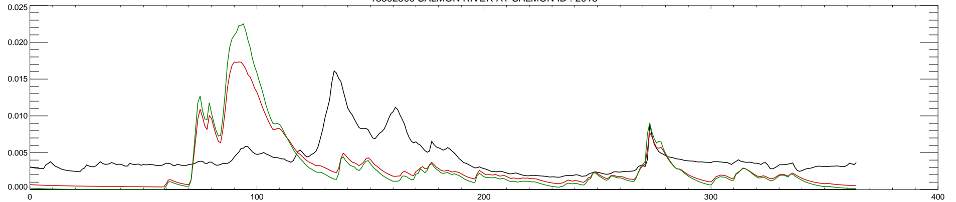
13302500 SALMON RIVER AT SALMON ID : 2013
