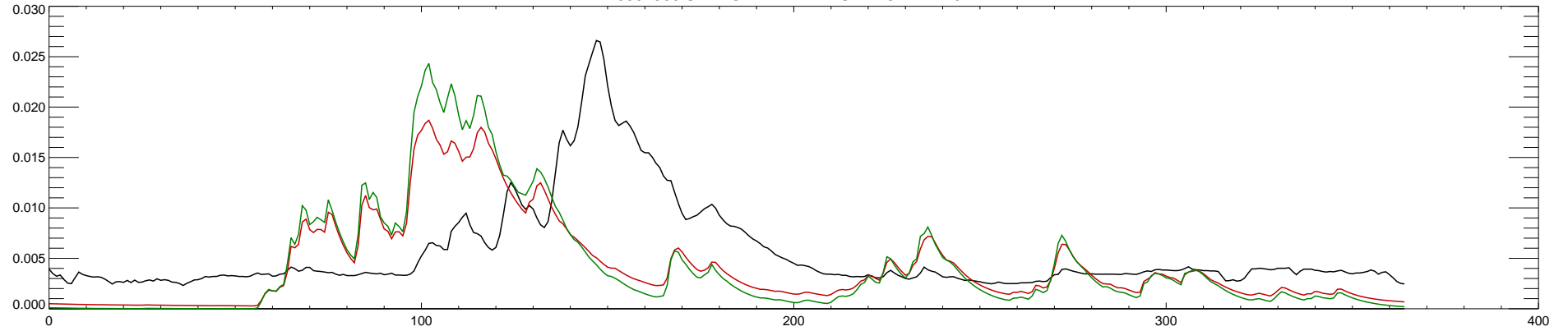
13302500 SALMON RIVER AT SALMON ID : 2015
