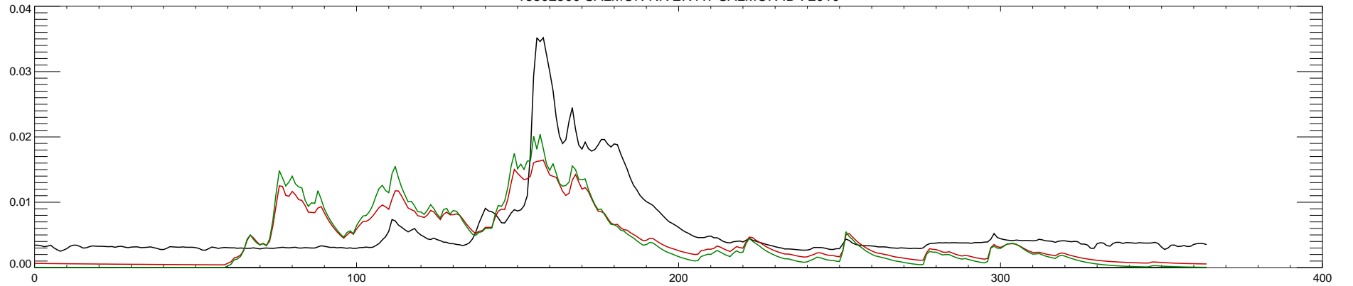
13302500 SALMON RIVER AT SALMON ID : 2010
