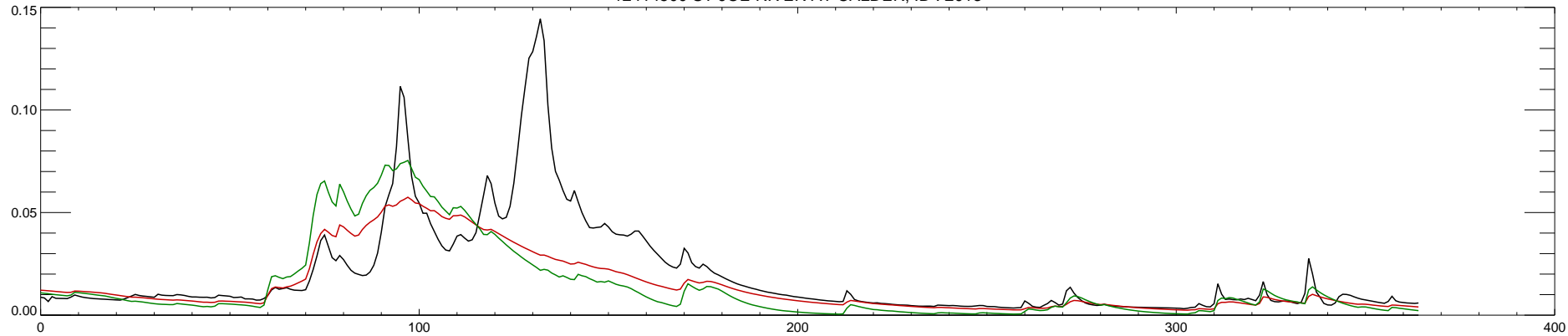
12414500 ST JOE RIVER AT CALDER, ID : 2013
