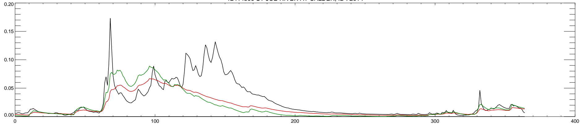
12414500 ST JOE RIVER AT CALDER, ID : 2015
