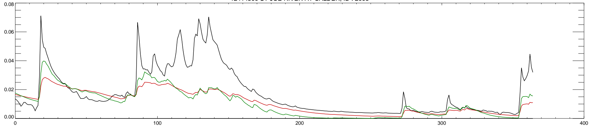
12414500 ST JOE RIVER AT CALDER, ID : 2006
