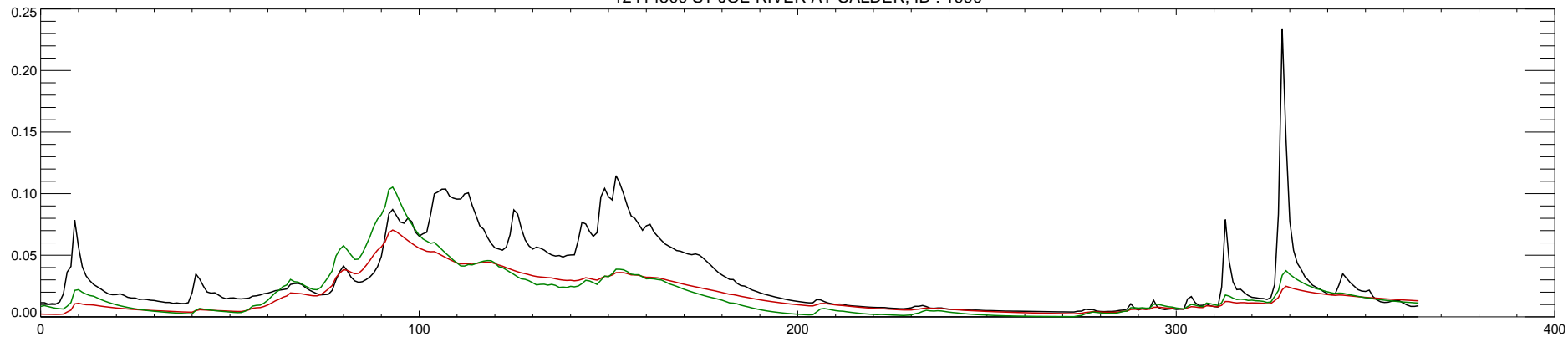
12414500 ST JOE RIVER AT CALDER, ID : 1991
