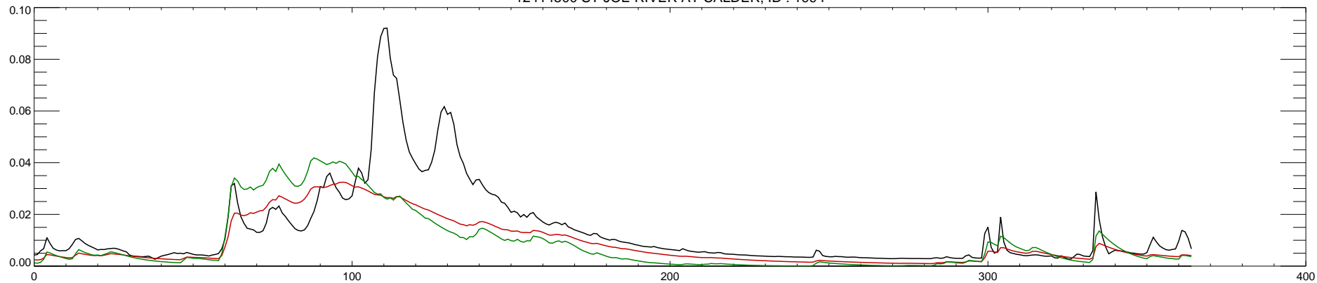
12414500 ST JOE RIVER AT CALDER, ID : 1995
