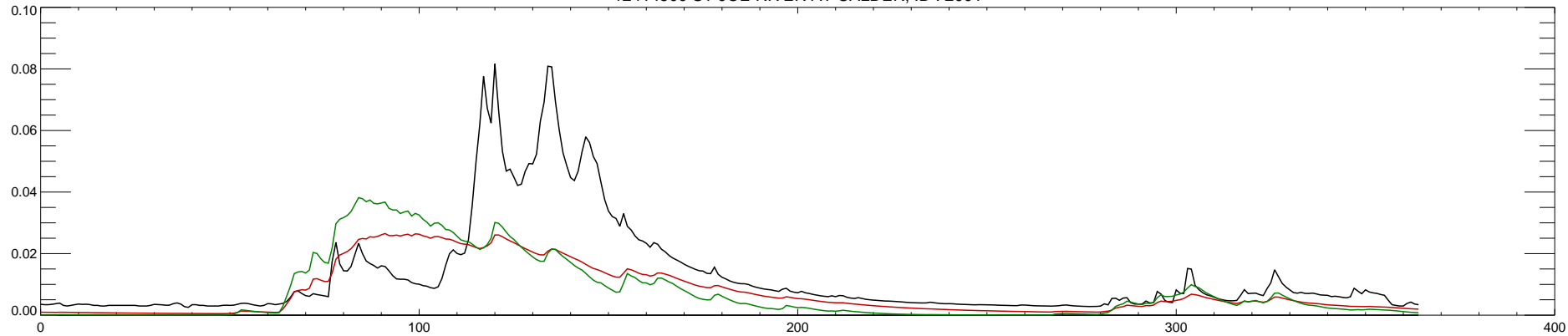
12414500 ST JOE RIVER AT CALDER, ID : 2001
