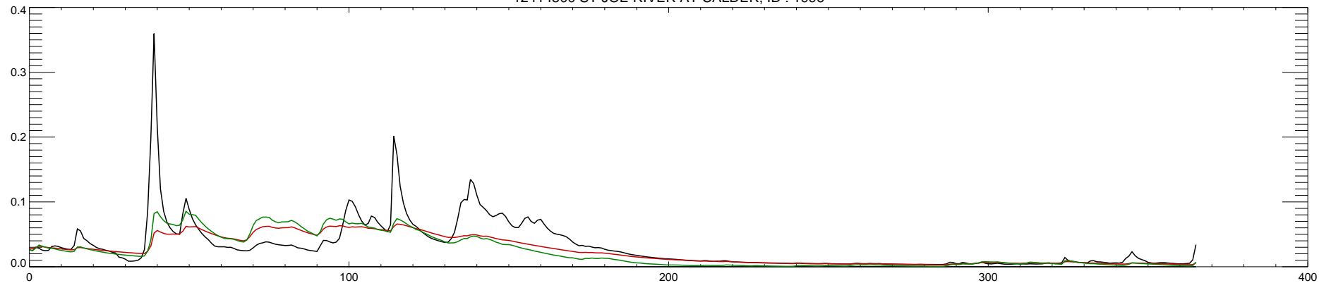
12414500 ST JOE RIVER AT CALDER, ID : 1997
