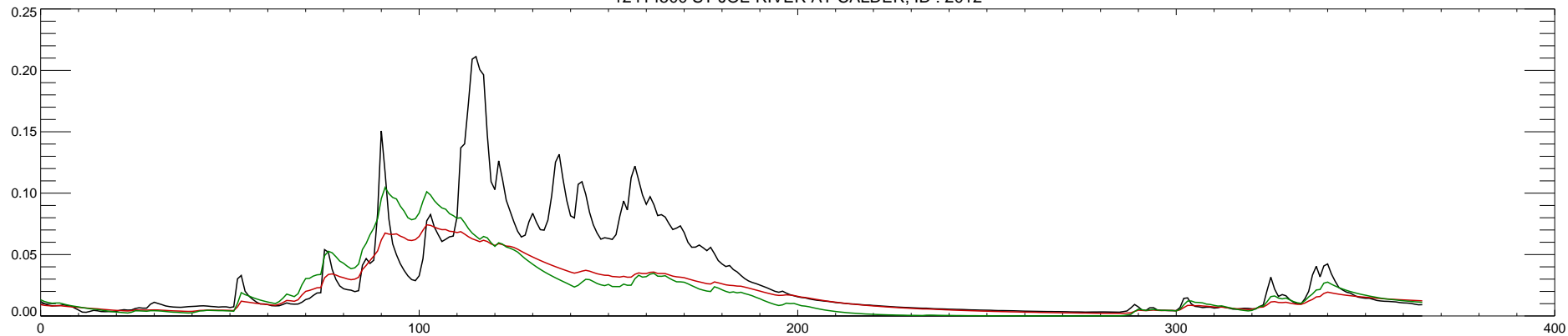
12414500 ST JOE RIVER AT CALDER, ID : 2013
