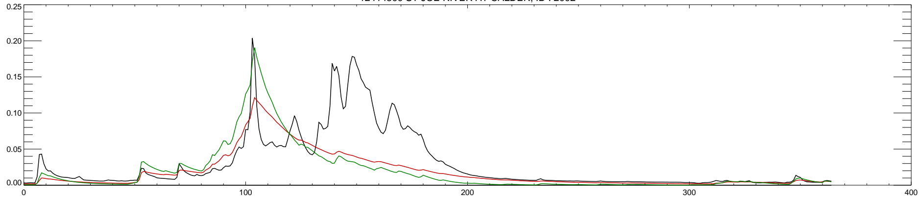
12414500 ST JOE RIVER AT CALDER, ID : 2003
