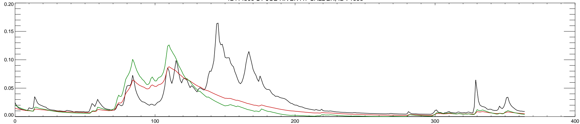
12414500 ST JOE RIVER AT CALDER, ID : 2000
