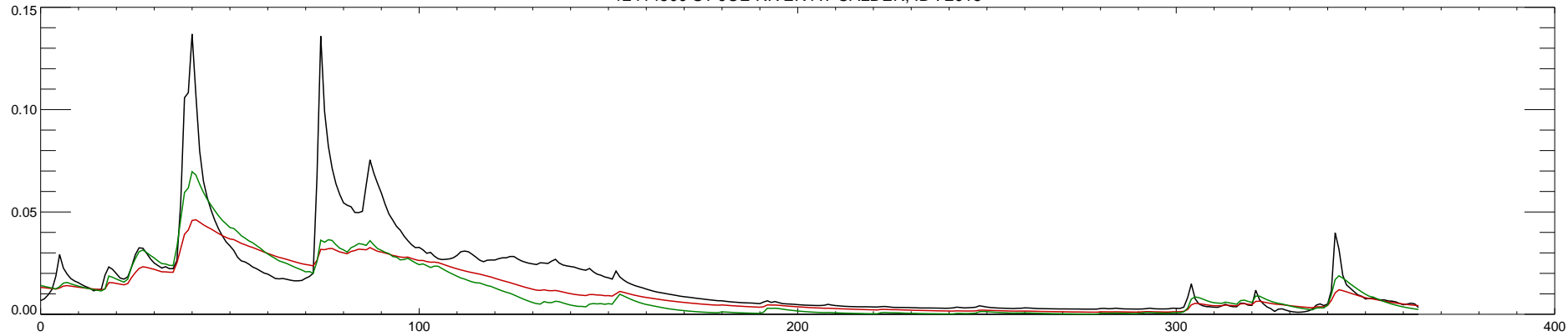
12414500 ST JOE RIVER AT CALDER, ID : 2016
