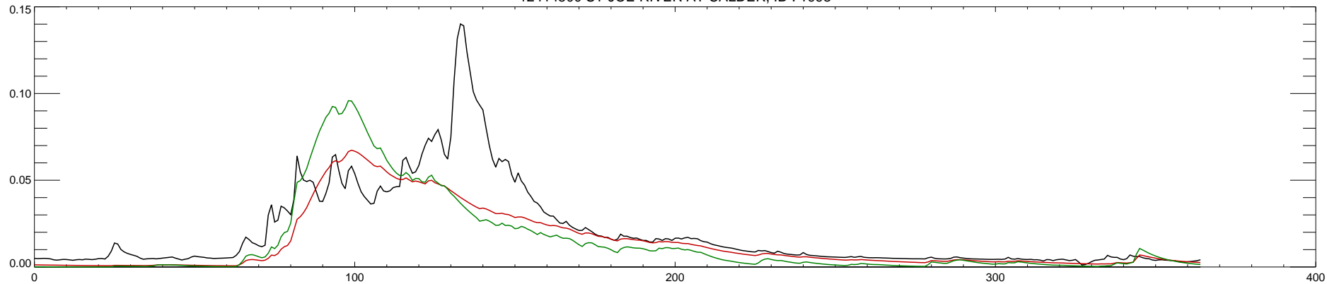
12414500 ST JOE RIVER AT CALDER, ID : 1994
