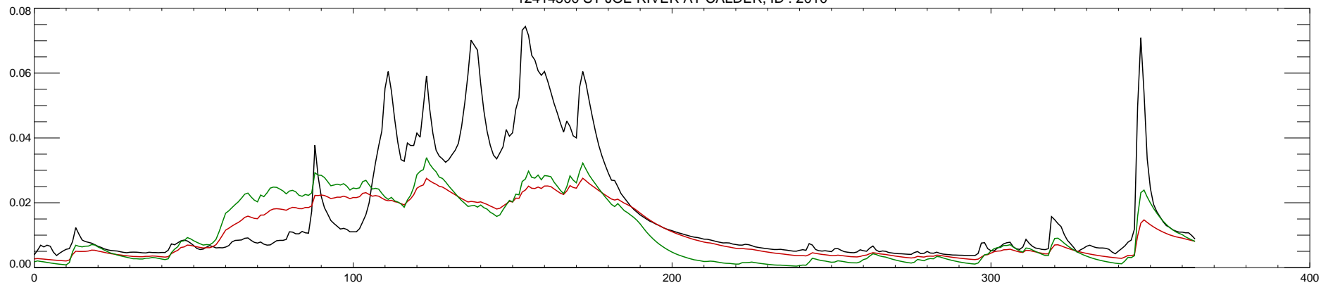
12414500 ST JOE RIVER AT CALDER, ID : 2010
