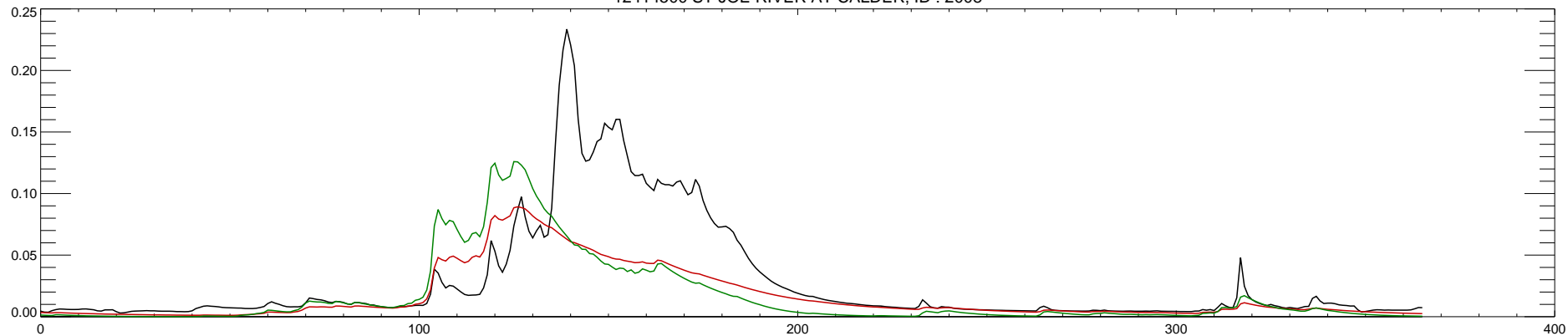
12414500 ST JOE RIVER AT CALDER, ID : 2009
