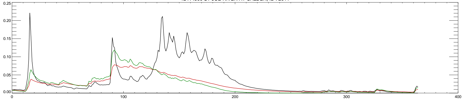
12414500 ST JOE RIVER AT CALDER, ID : 2012
