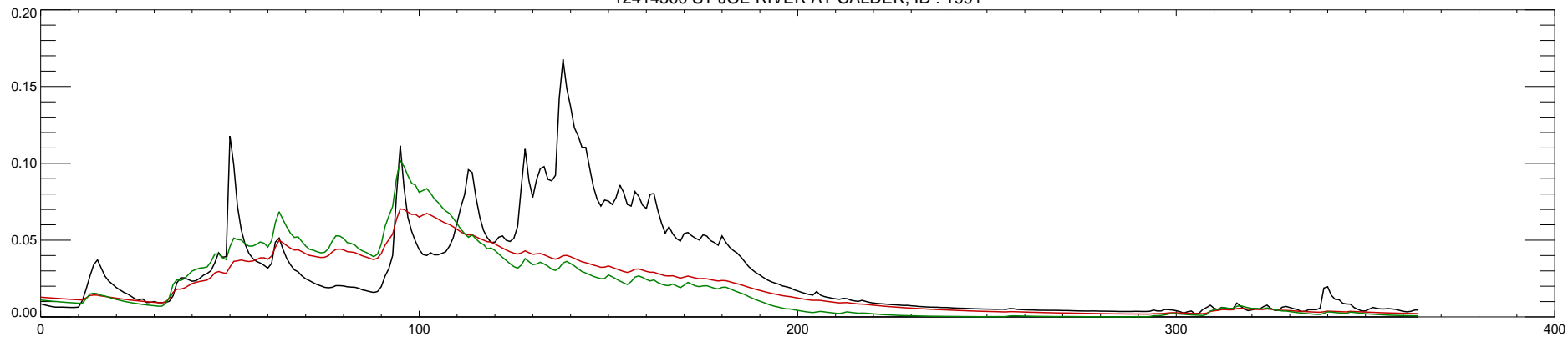
12414500 ST JOE RIVER AT CALDER, ID : 1992
