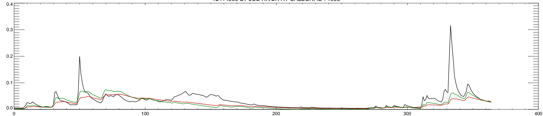
12414500 ST JOE RIVER AT CALDER, ID : 1995
