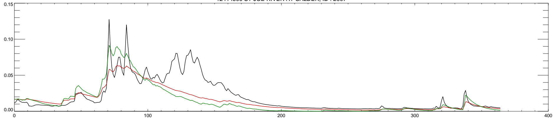
12414500 ST JOE RIVER AT CALDER, ID : 2007
