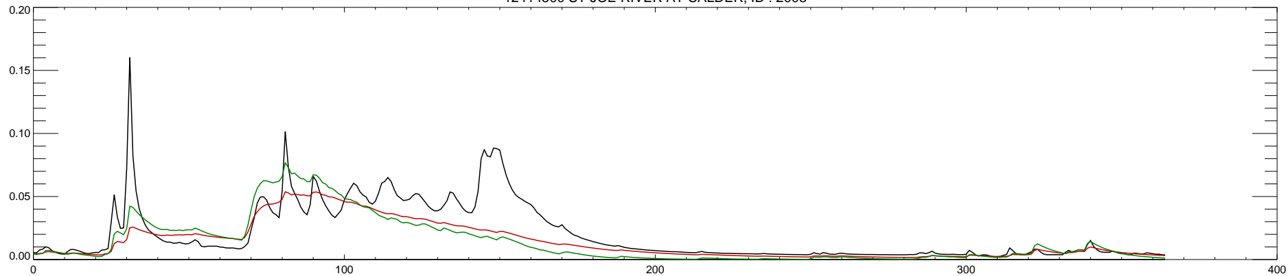
12414500 ST JOE RIVER AT CALDER, ID : 2004
