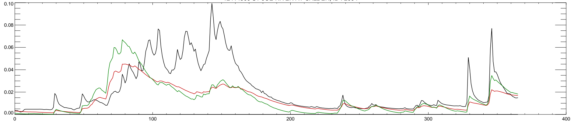
12414500 ST JOE RIVER AT CALDER, ID : 2004
