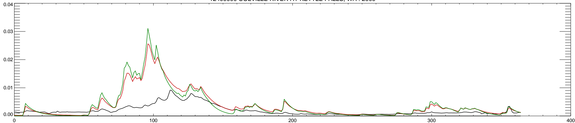
12409000 COLVILLE RIVER AT KETTLE FALLS, WA : 2010
