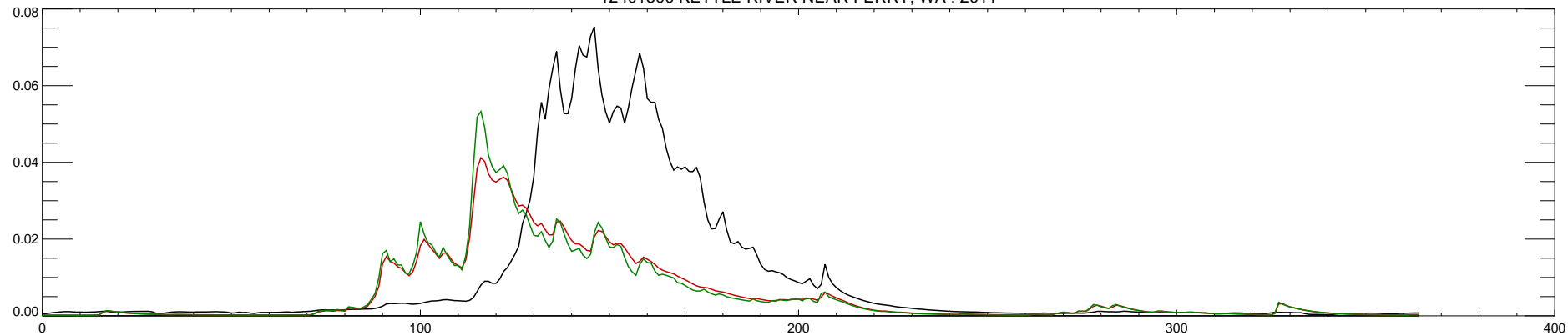
12401500 KETTLE RIVER NEAR FERRY, WA : 2012
