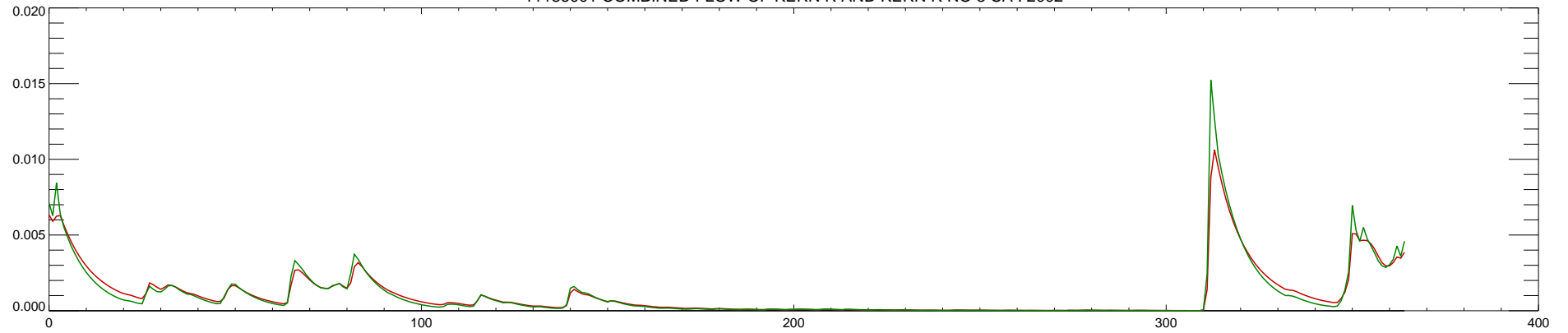
11186001 COMBINED FLOW OF KERN R AND KERN R NO 3 CA : 2003
