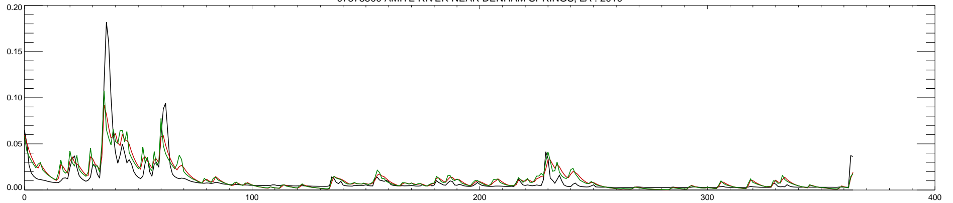
07378500 AMITE RIVER NEAR DENHAM SPRINGS, LA : 2010
