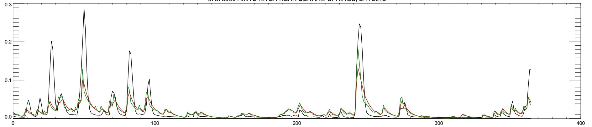
07378500 AMITE RIVER NEAR DENHAM SPRINGS, LA : 2013
