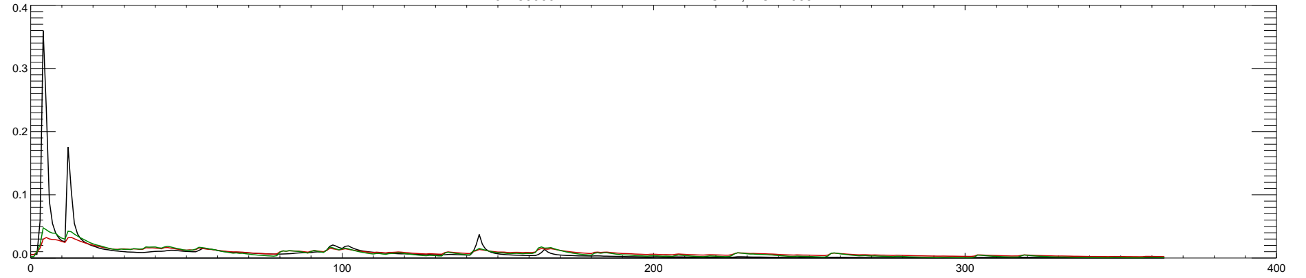
07189000 ELK RIVER NEAR TIFF CITY, MO : 2006
