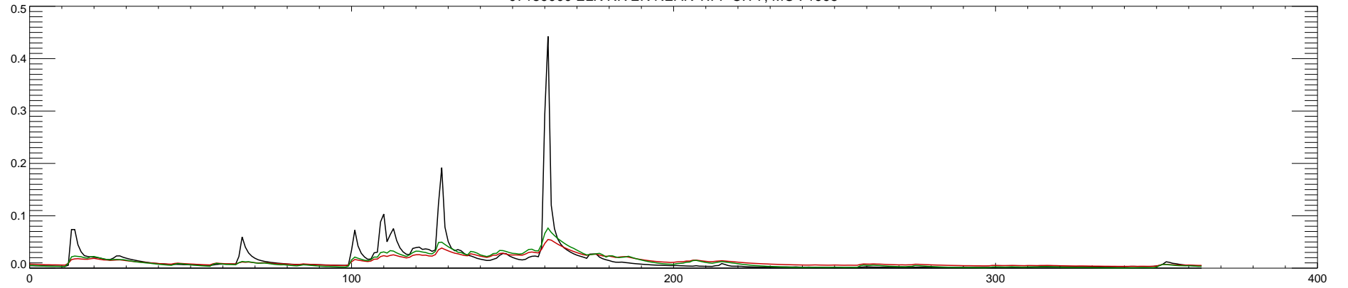
07189000 ELK RIVER NEAR TIFF CITY, MO : 1995
