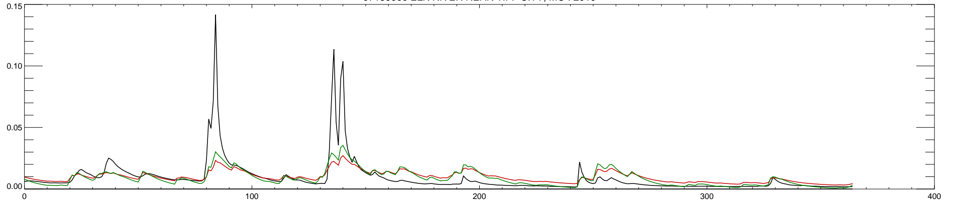
07189000 ELK RIVER NEAR TIFF CITY, MO : 2010
