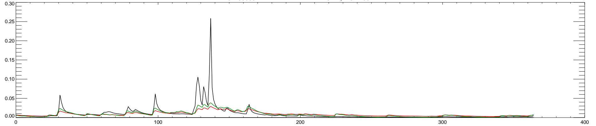
07189000 ELK RIVER NEAR TIFF CITY, MO : 2003
