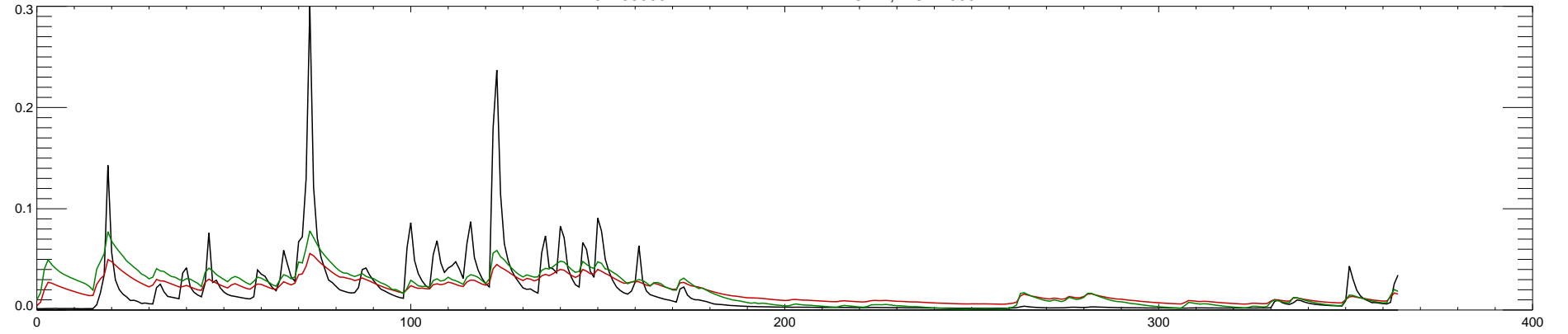
07189000 ELK RIVER NEAR TIFF CITY, MO : 1991
