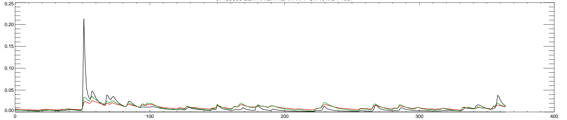
07189000 ELK RIVER NEAR TIFF CITY, MO : 1998
