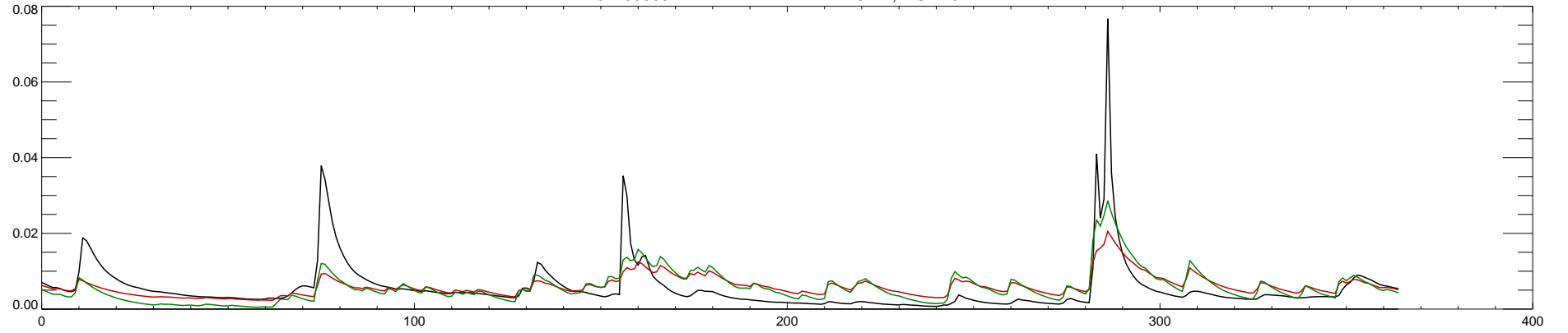
07189000 ELK RIVER NEAR TIFF CITY, MO : 2015
