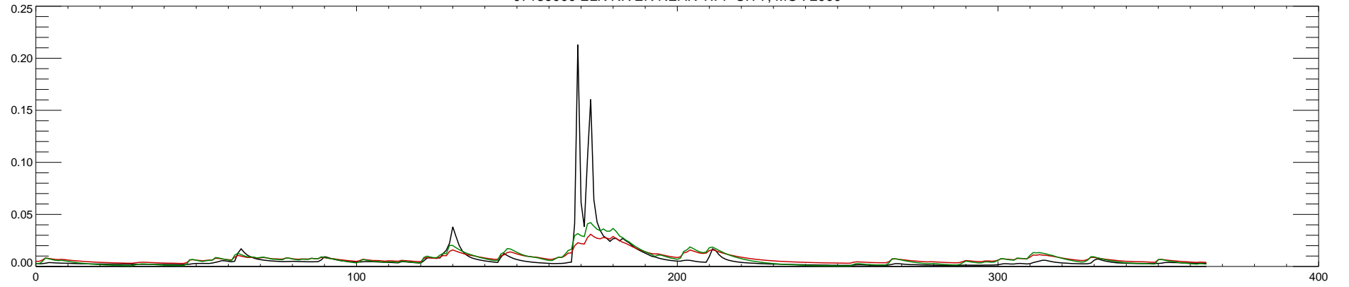
07189000 ELK RIVER NEAR TIFF CITY, MO : 2001
