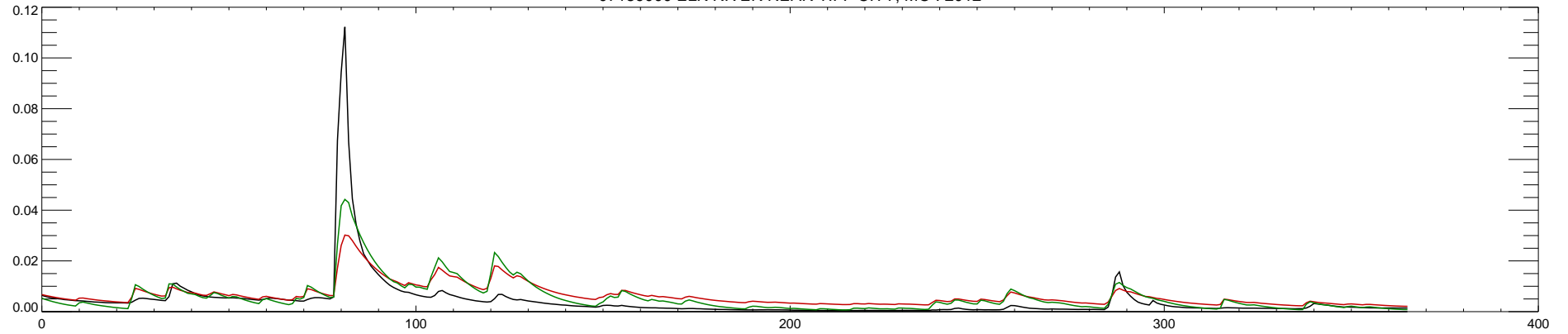
07189000 ELK RIVER NEAR TIFF CITY, MO : 2013
