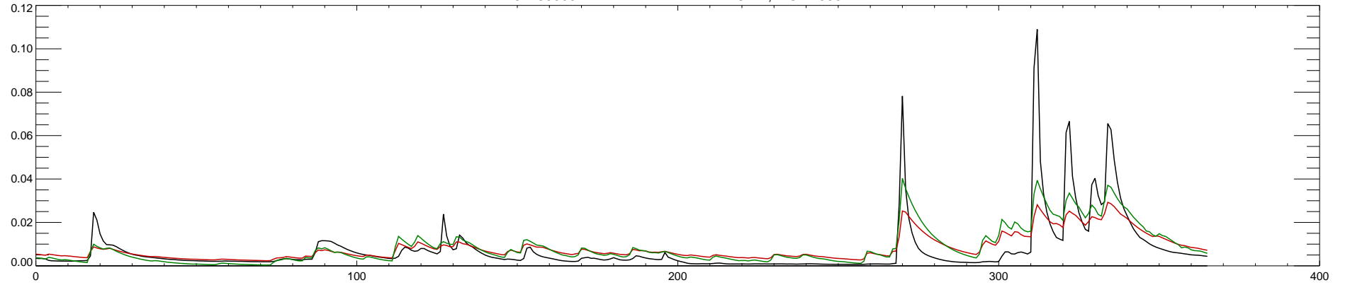
07189000 ELK RIVER NEAR TIFF CITY, MO : 1997
