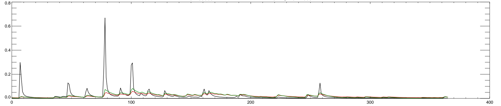
07189000 ELK RIVER NEAR TIFF CITY, MO : 2009
