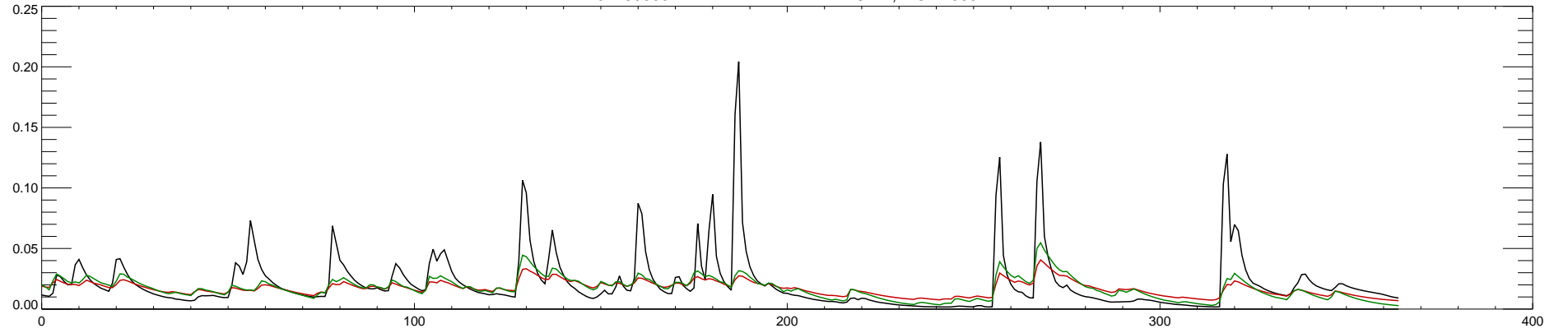
07189000 ELK RIVER NEAR TIFF CITY, MO : 1994
