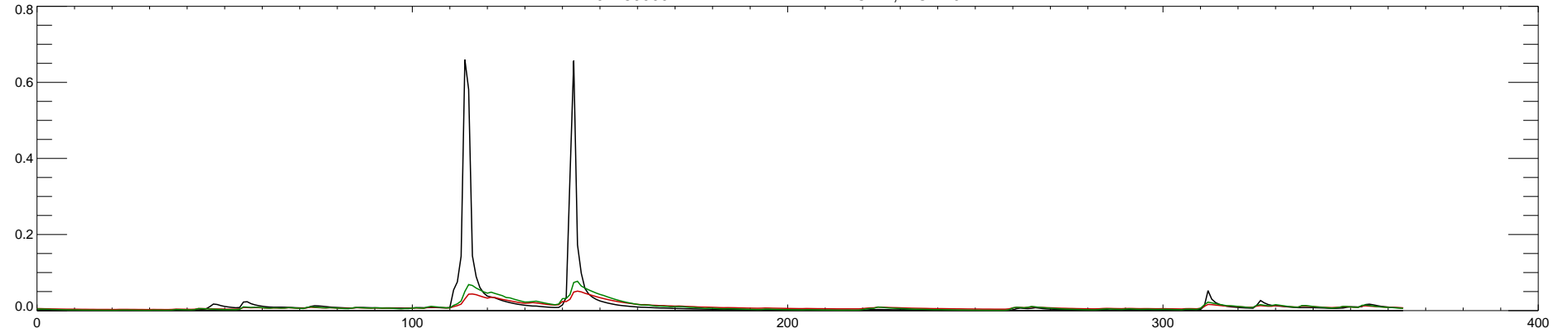
07189000 ELK RIVER NEAR TIFF CITY, MO : 2012
