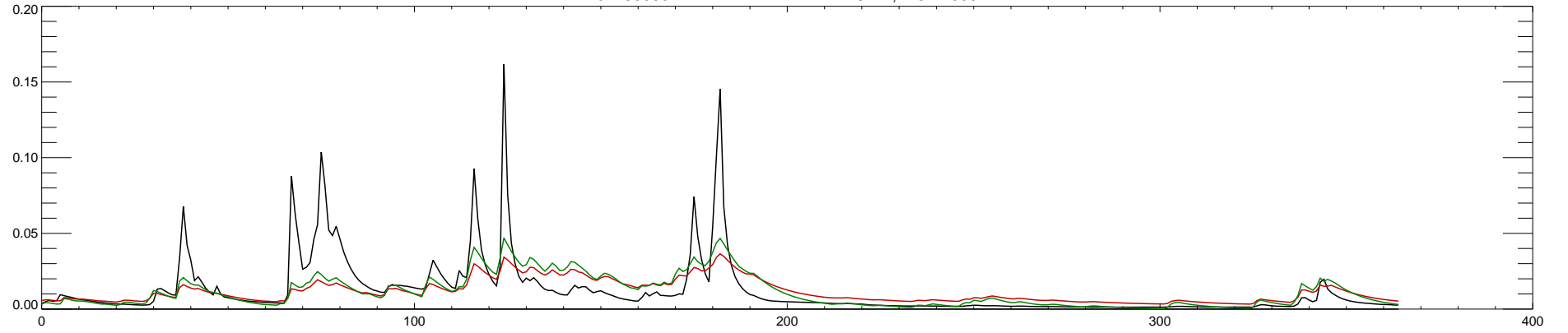
07189000 ELK RIVER NEAR TIFF CITY, MO : 2000
