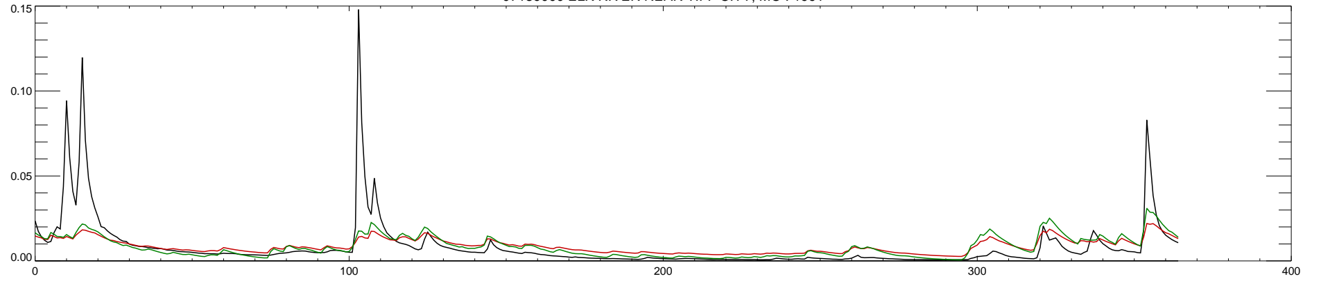
07189000 ELK RIVER NEAR TIFF CITY, MO : 1992
