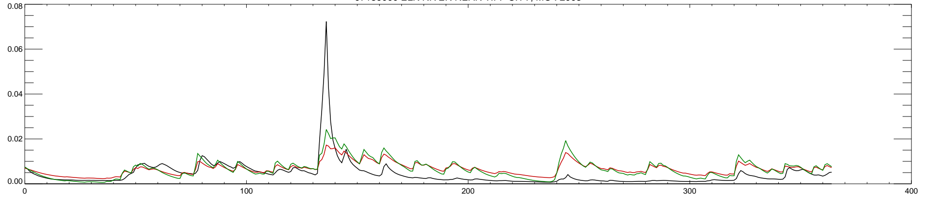
07189000 ELK RIVER NEAR TIFF CITY, MO : 2004
