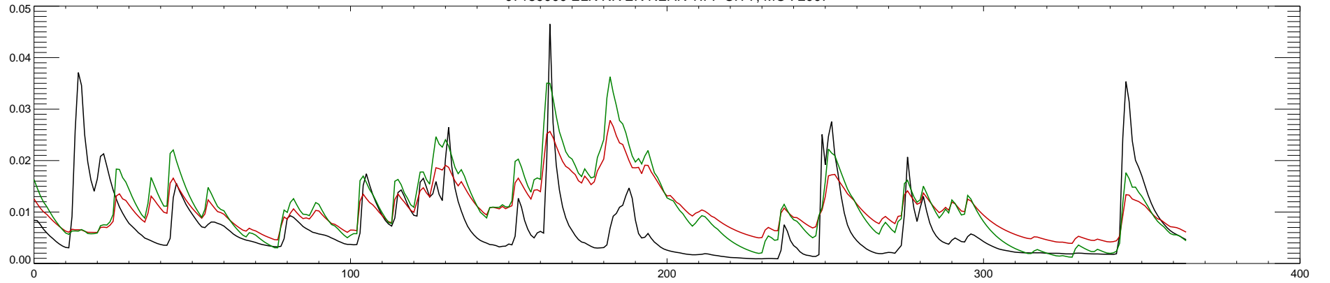
07189000 ELK RIVER NEAR TIFF CITY, MO : 2007
