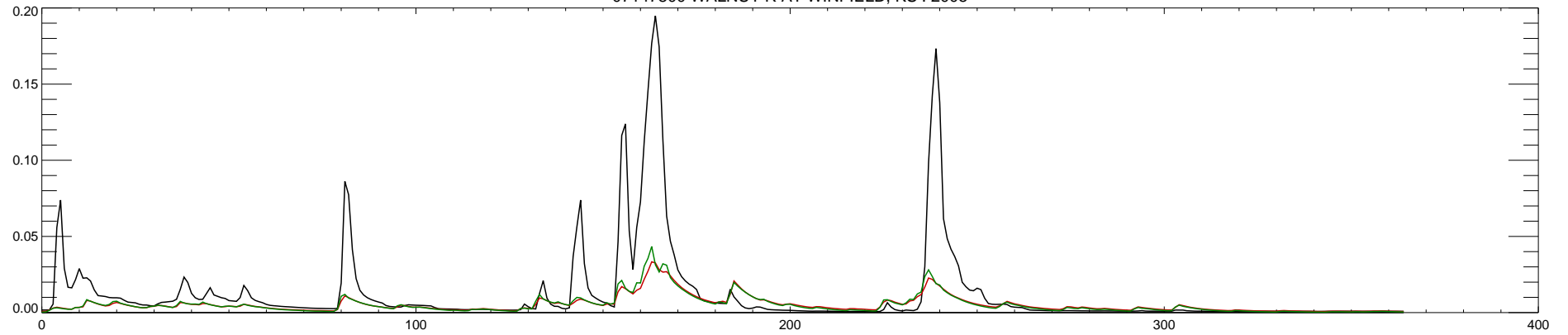
07147800 WALNUT R AT WINFIELD, KS : 2006
