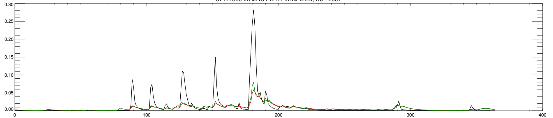
07147800 WALNUT R AT WINFIELD, KS : 2007
