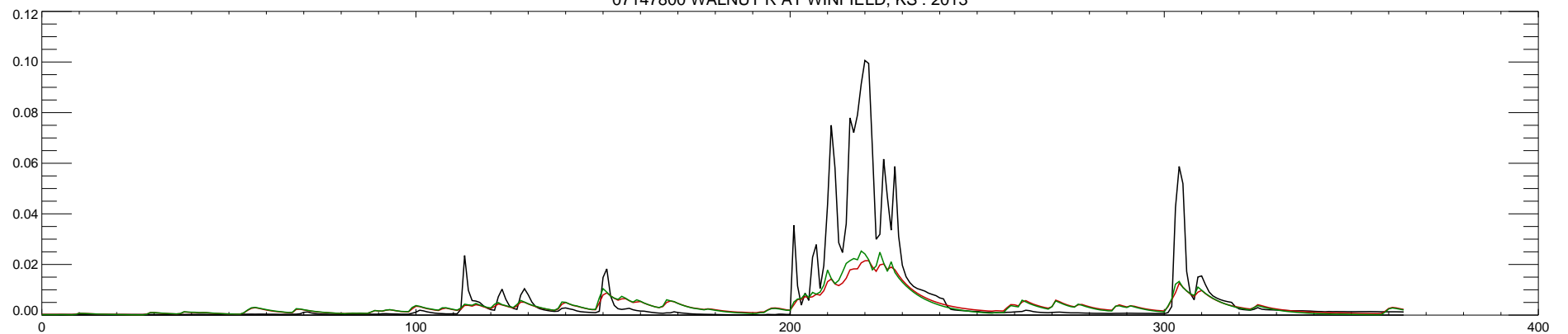
07147800 WALNUT R AT WINFIELD, KS : 2013
