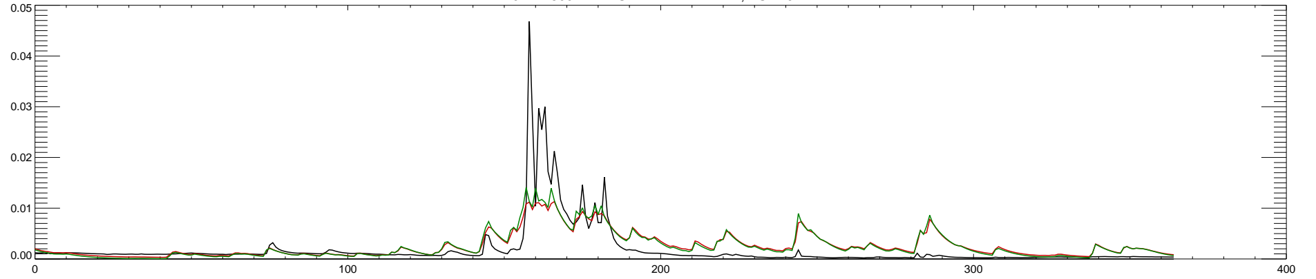
07147800 WALNUT R AT WINFIELD, KS : 2015
