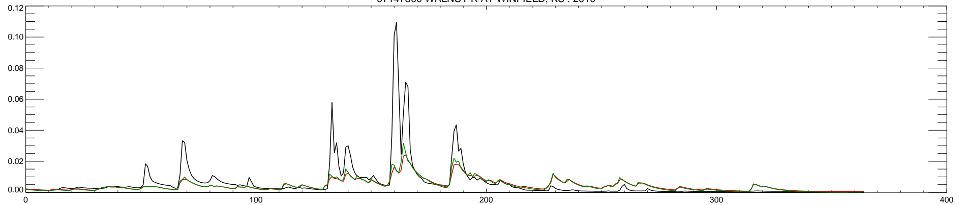
07147800 WALNUT R AT WINFIELD, KS : 2010
