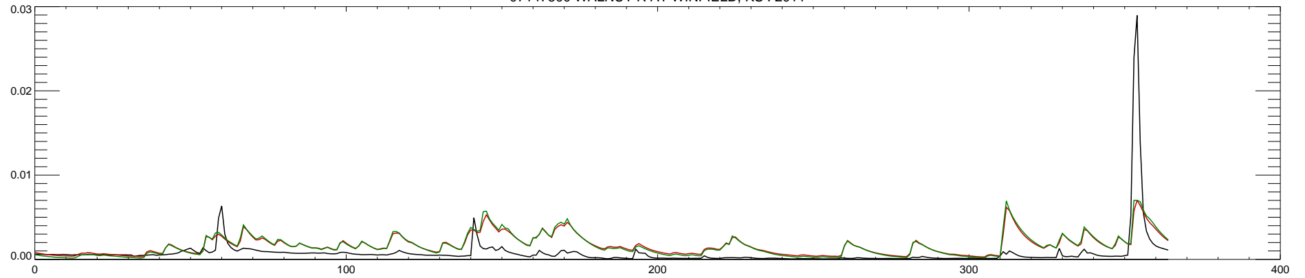
07147800 WALNUT R AT WINFIELD, KS : 2012
