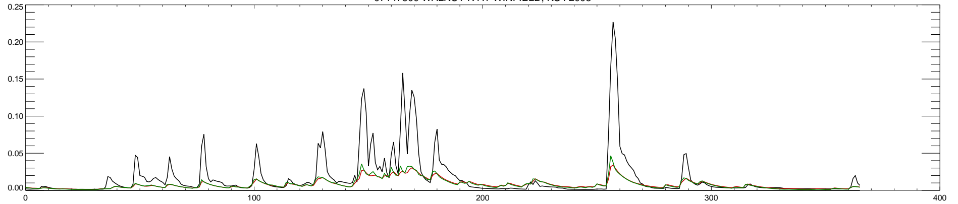
07147800 WALNUT R AT WINFIELD, KS : 2009
