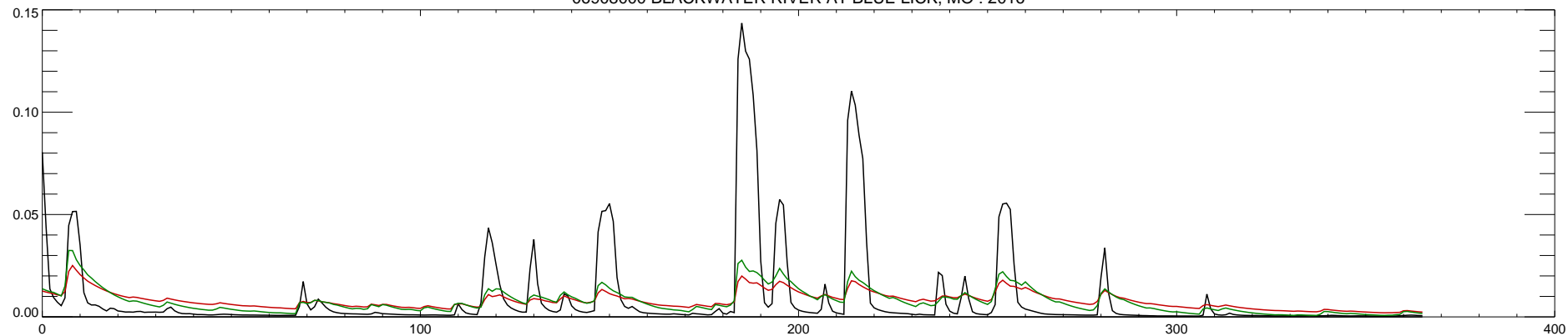
06908000 BLACKWATER RIVER AT BLUE LICK, MO : 2016
