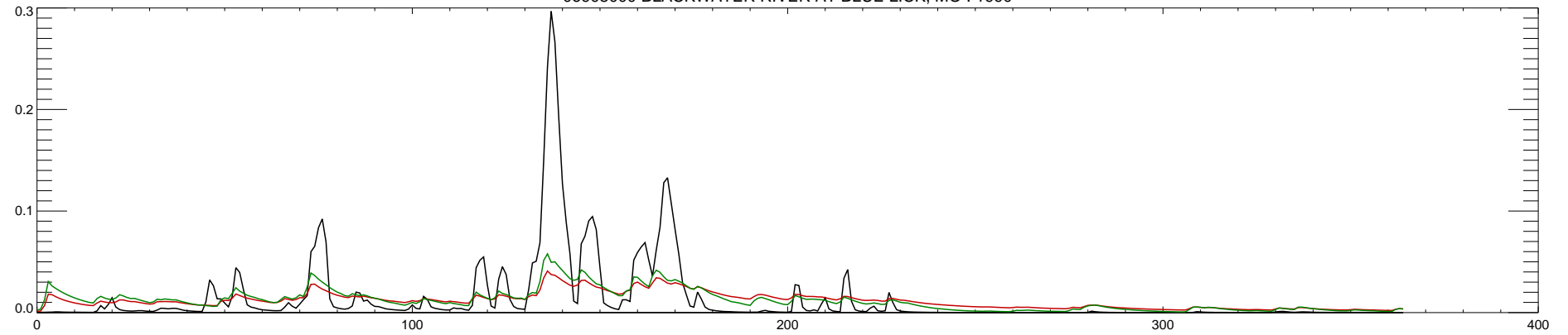
06908000 BLACKWATER RIVER AT BLUE LICK, MO : 1991
