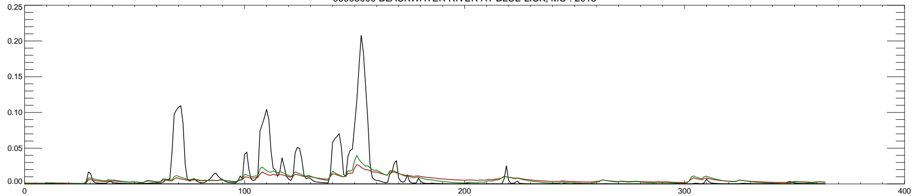
06908000 BLACKWATER RIVER AT BLUE LICK, MO : 2013
