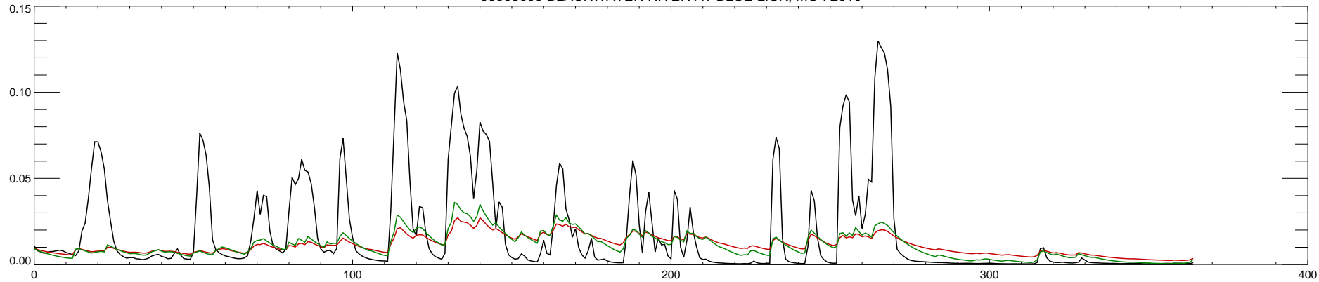
06908000 BLACKWATER RIVER AT BLUE LICK, MO : 2010
