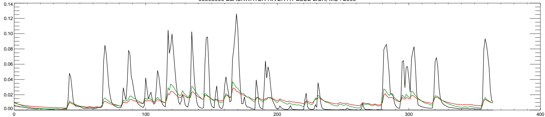
06908000 BLACKWATER RIVER AT BLUE LICK, MO : 2010
