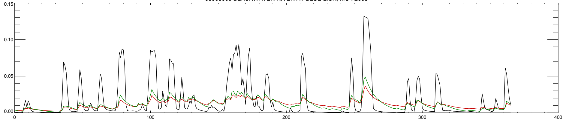
06908000 BLACKWATER RIVER AT BLUE LICK, MO : 2009
