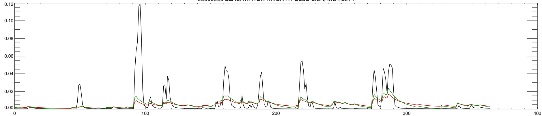
06908000 BLACKWATER RIVER AT BLUE LICK, MO : 2015
