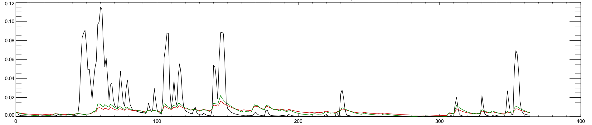
06908000 BLACKWATER RIVER AT BLUE LICK, MO : 2012
