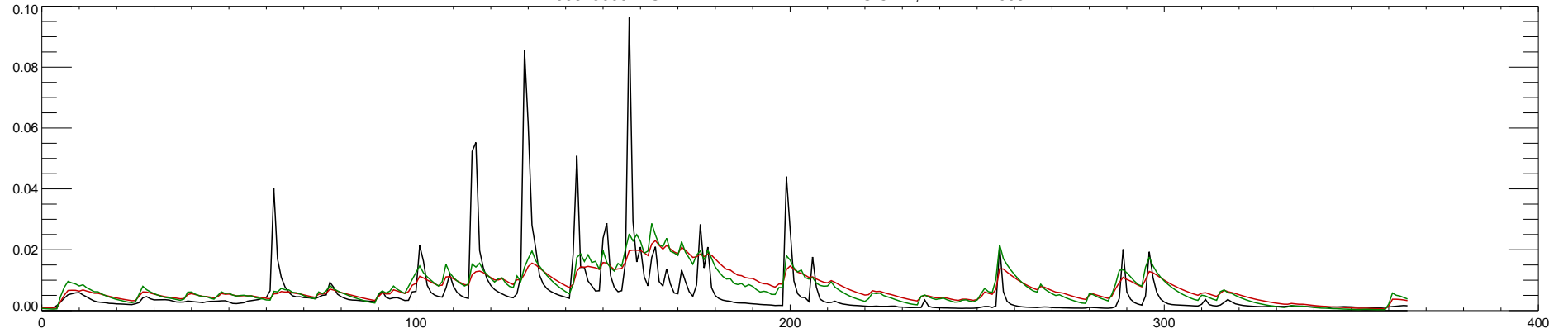
06815000 BIG NEMAHA RIVER AT FALLS CITY, NEBR. : 2009
