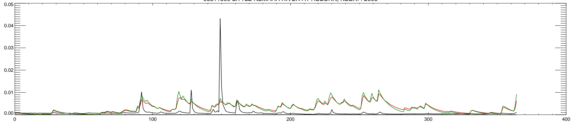
06811500 LITTLE NEMAHA RIVER AT AUBURN, NEBR. : 2007
