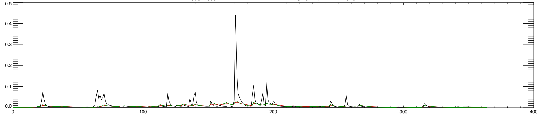
06811500 LITTLE NEMAHA RIVER AT AUBURN, NEBR. : 2010
