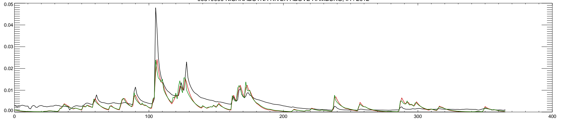
06810000 NISHNABOTNA RIVER ABOVE HAMBURG, IA : 2013
