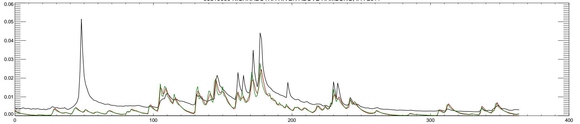
06810000 NISHNABOTNA RIVER ABOVE HAMBURG, IA : 2012
