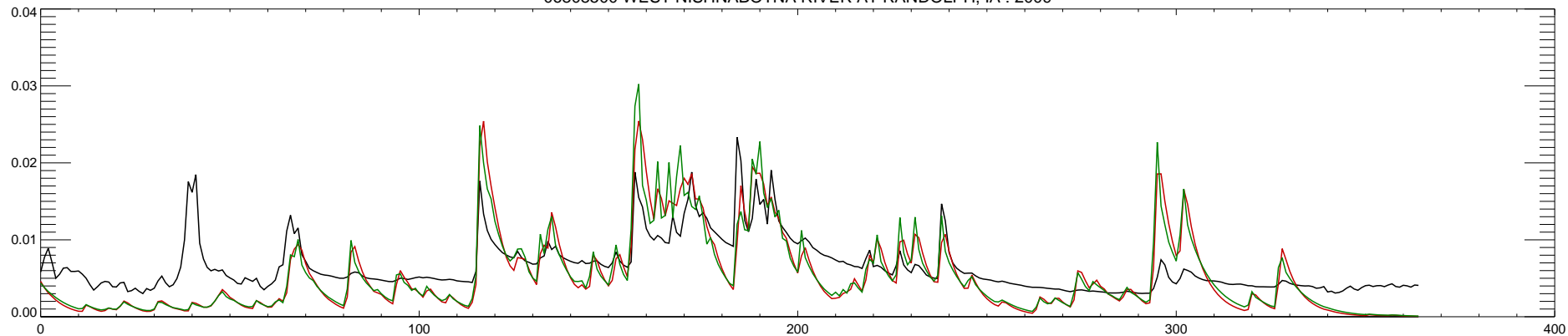
06808500 WEST NISHNABOTNA RIVER AT RANDOLPH, IA : 2010
