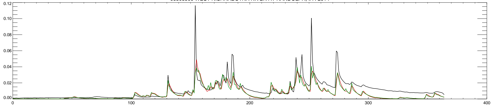
06808500 WEST NISHNABOTNA RIVER AT RANDOLPH, IA : 2015
