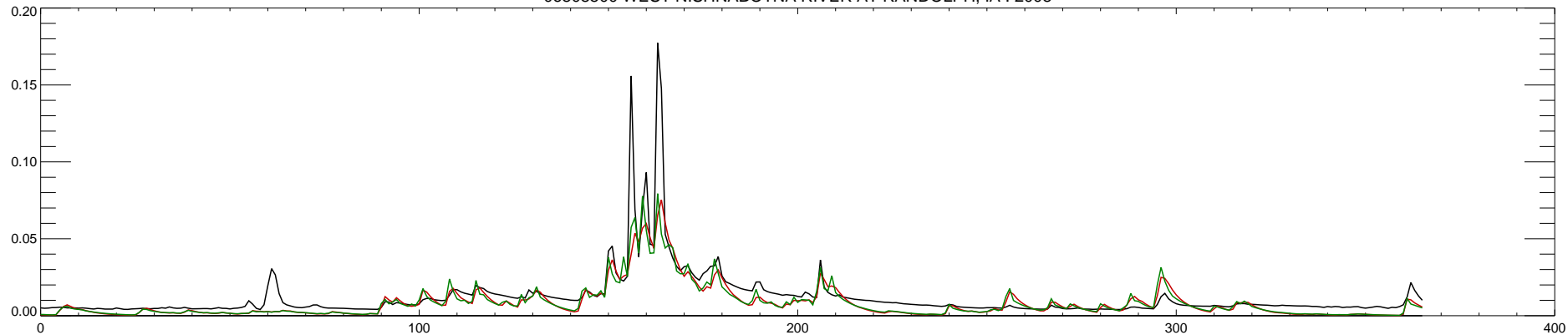
06808500 WEST NISHNABOTNA RIVER AT RANDOLPH, IA : 2009
