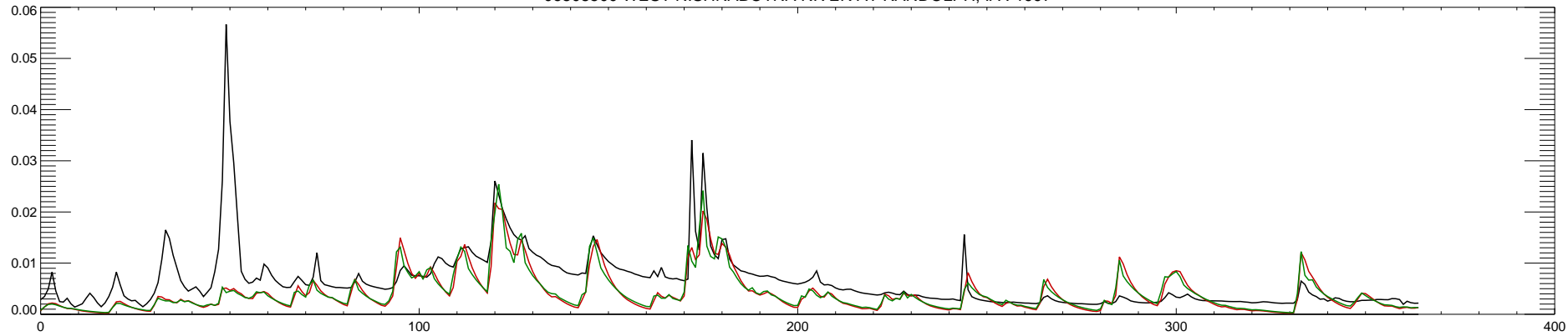
06808500 WEST NISHNABOTNA RIVER AT RANDOLPH, IA : 1998
