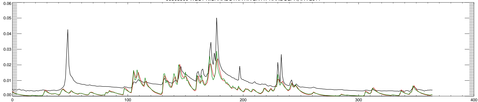
06808500 WEST NISHNABOTNA RIVER AT RANDOLPH, IA : 2012
