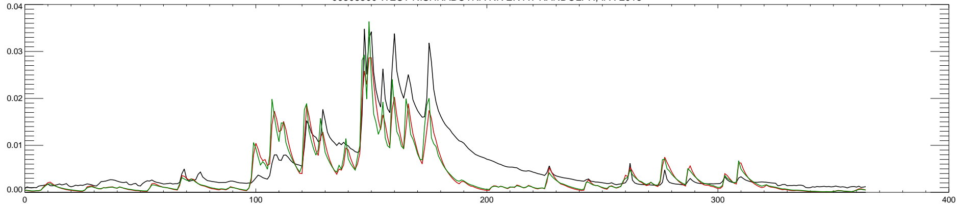
06808500 WEST NISHNABOTNA RIVER AT RANDOLPH, IA : 2013
