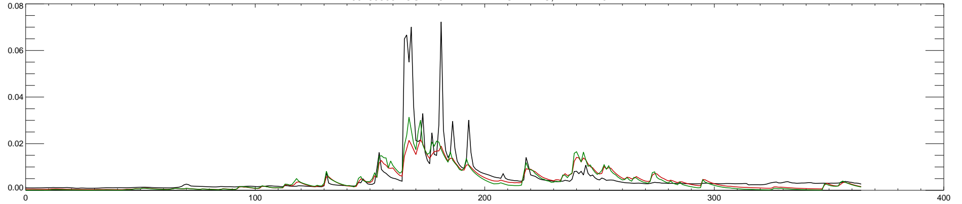
06799500 LOGAN CREEK NEAR UEHLING, NEBR. : 2015
