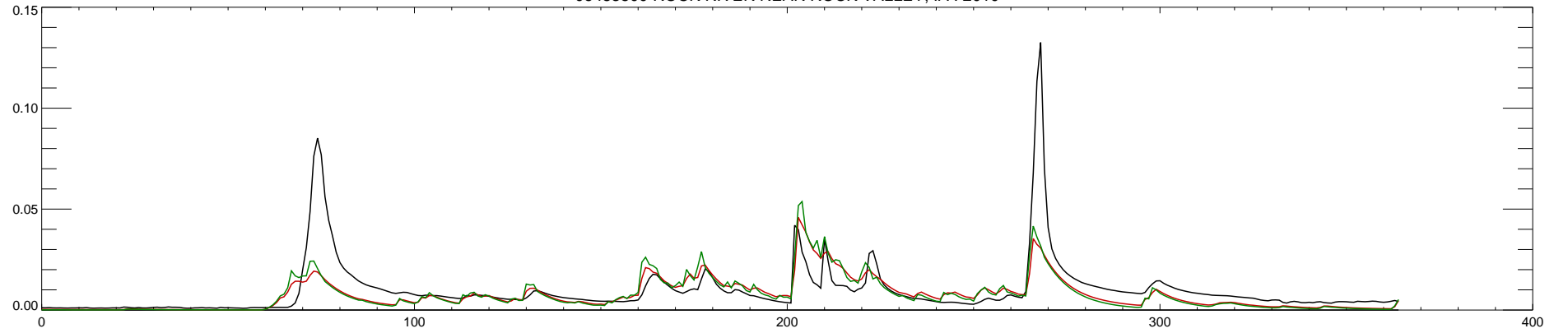
06483500 ROCK RIVER NEAR ROCK VALLEY, IA : 2010
