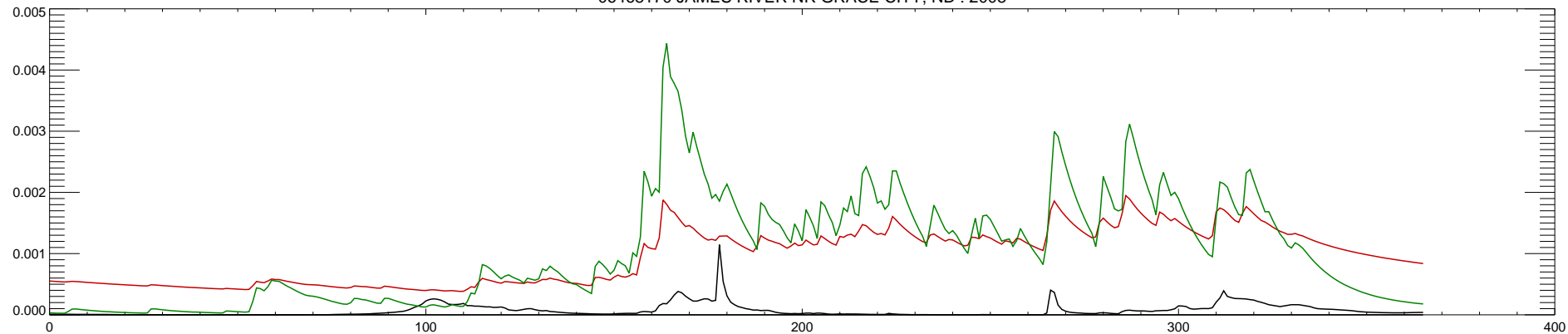
06468170 JAMES RIVER NR GRACE CITY, ND : 2009
