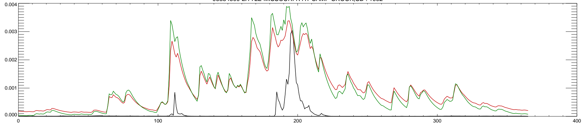
06334500 LITTLE MISSOURI R AT CAMP CROOK,SD : 1992
