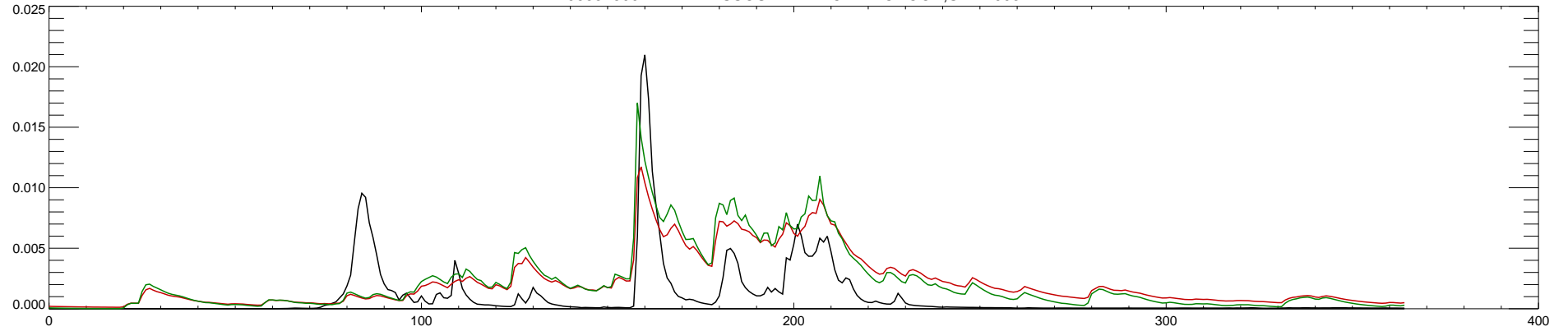
06334500 LITTLE MISSOURI R AT CAMP CROOK,SD : 1994
