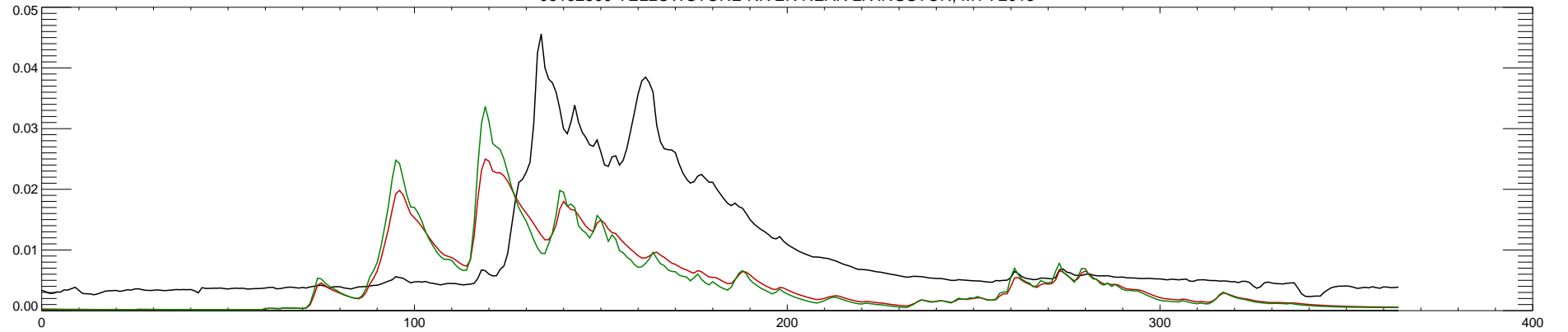
06192500 YELLOWSTONE RIVER NEAR LIVINGSTON, MT : 2013
