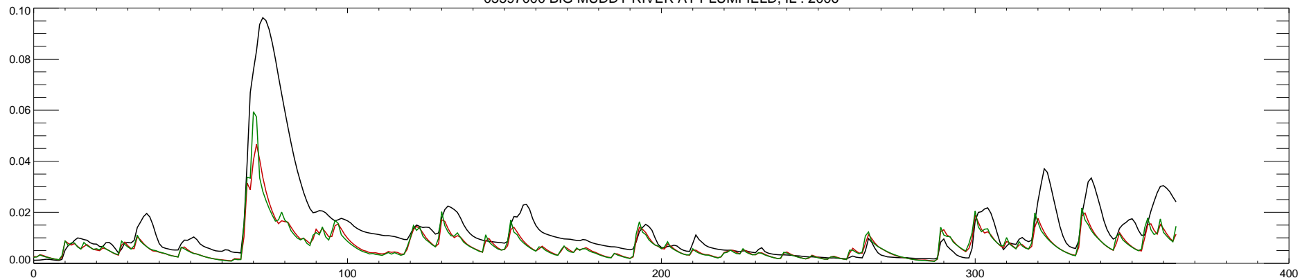
05597000 BIG MUDDY RIVER AT PLUMFIELD, IL : 2007
