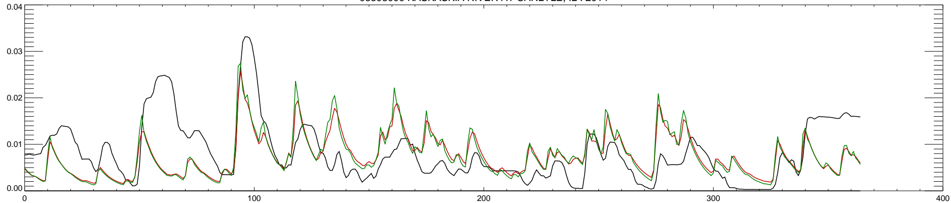
05593000 KASKASKIA RIVER AT CARLYLE, IL : 2015
