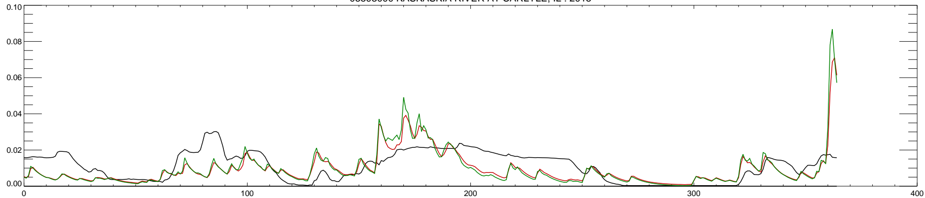
05593000 KASKASKIA RIVER AT CARLYLE, IL : 2016
