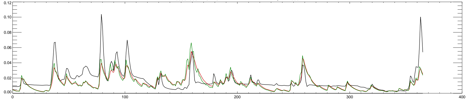
05592500 KASKASKIA RIVER AT VANDALIA, IL : 2009
