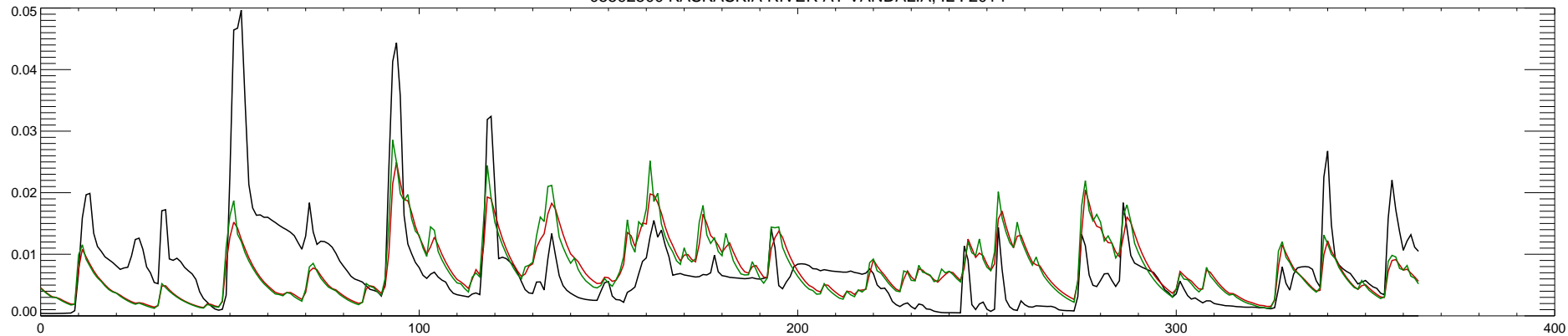
05592500 KASKASKIA RIVER AT VANDALIA, IL : 2015
