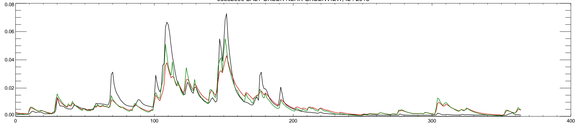
05582000 SALT CREEK NEAR GREENVIEW, IL : 2013
