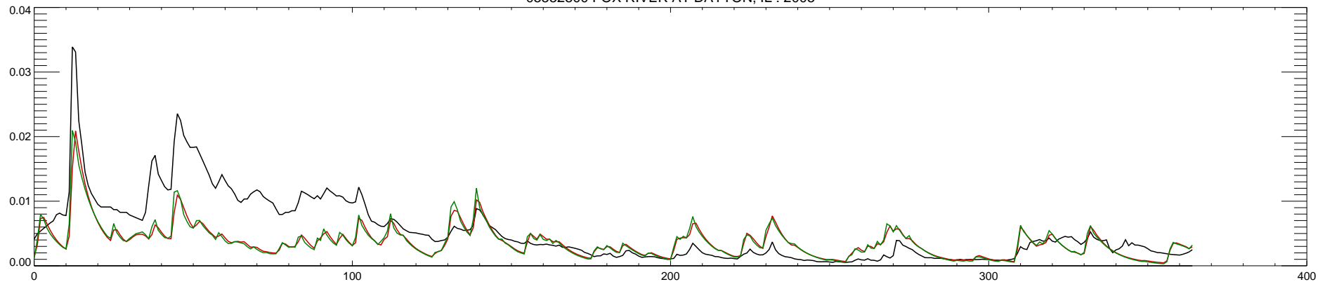
0552500 FOX RIVER AT DAYTON, IL : 2006
