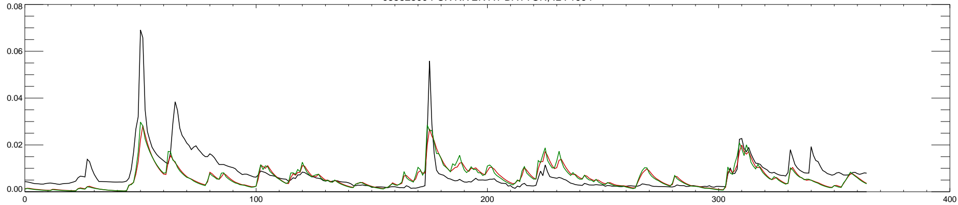
0552500 FOX RIVER AT DAYTON, IL : 1995
