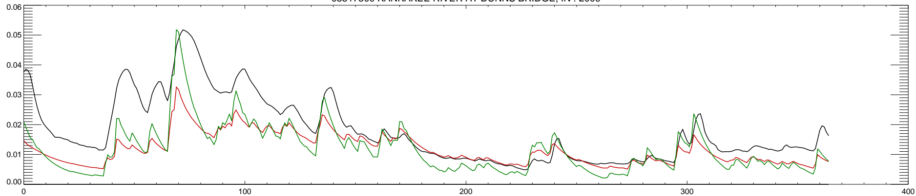
05517500 KANKAKEE RIVER AT DUNNS BRIDGE, IN : 2010
