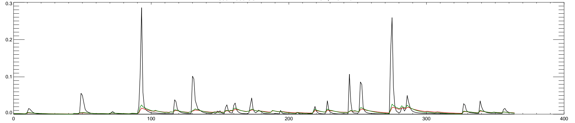
05514500 CUIVRE RIVER NEAR TROY, MO : 2015
