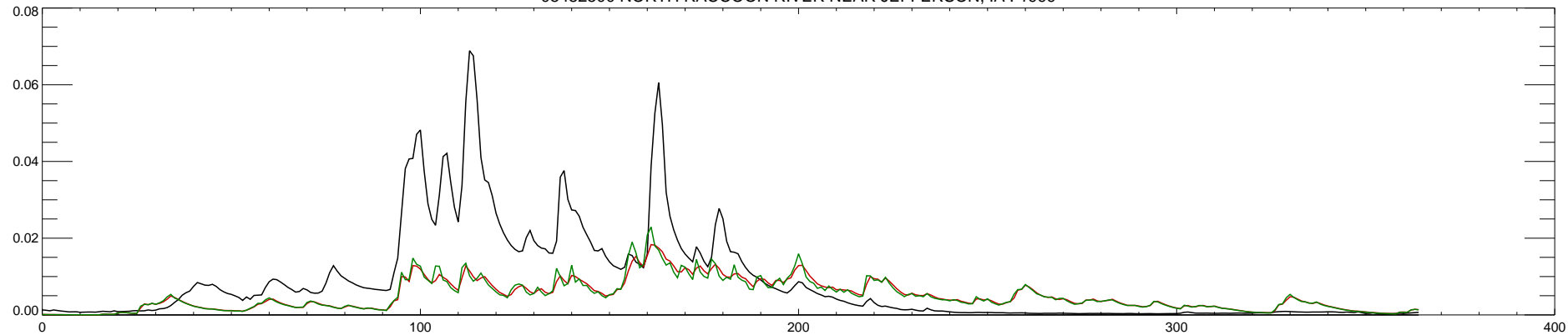
05482500 NORTH RACCOON RIVER NEAR JEFFERSON, IA : 2000
