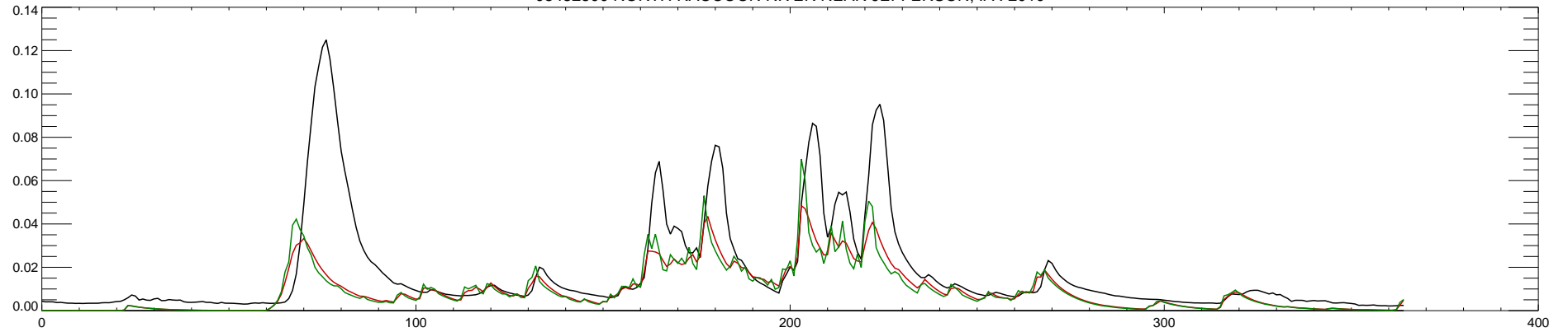
05482500 NORTH RACCOON RIVER NEAR JEFFERSON, IA : 2010
