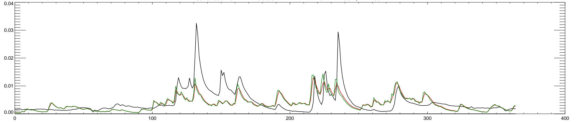
05482500 NORTH RACCOON RIVER NEAR JEFFERSON, IA : 2003
