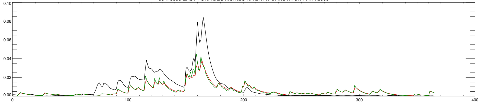
05479000 EAST FORK DES MOINES RIVER AT DAKOTA CITY, IA : 2009
