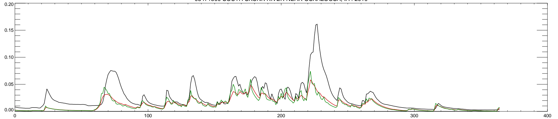
05471500 SOUTH SKUNK RIVER NEAR OSKALOOSA, IA : 2010
