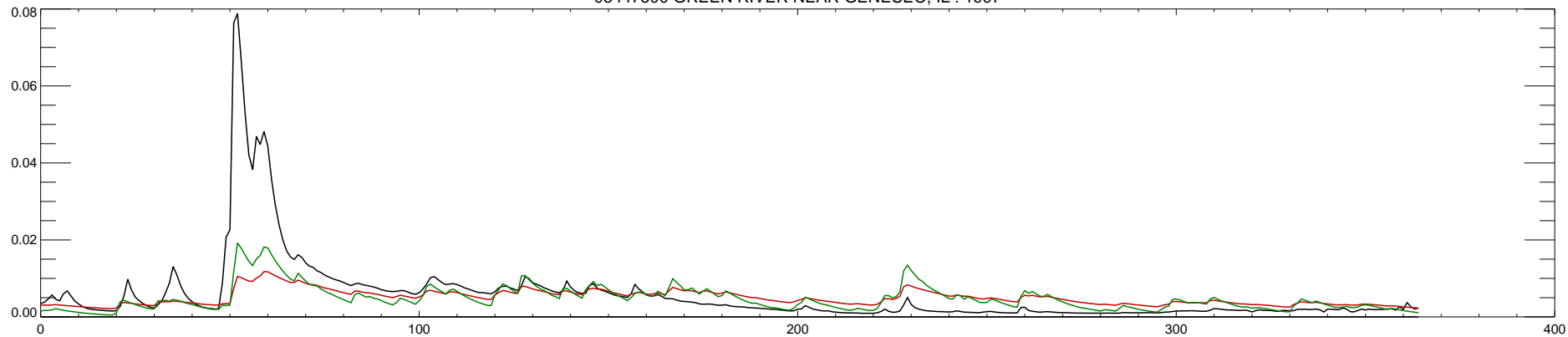
05447500 GREEN RIVER NEAR GENESEO, IL : 1998
