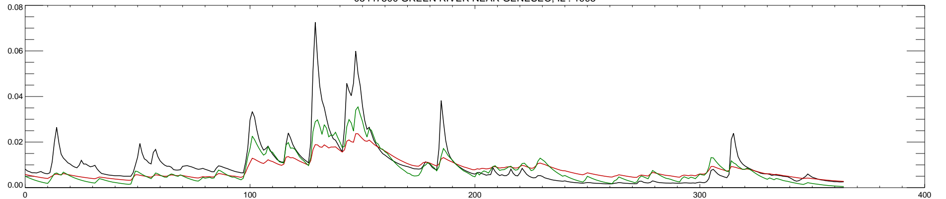
05447500 GREEN RIVER NEAR GENESEO, IL : 1995
