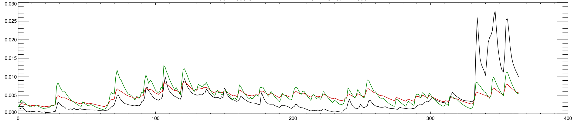
05447500 GREEN RIVER NEAR GENESEO, IL : 2007
