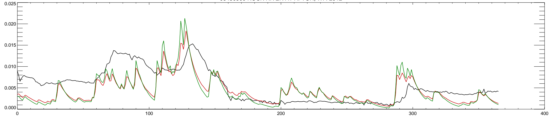
05430500 ROCK RIVER AT AFTON, WI : 2013
