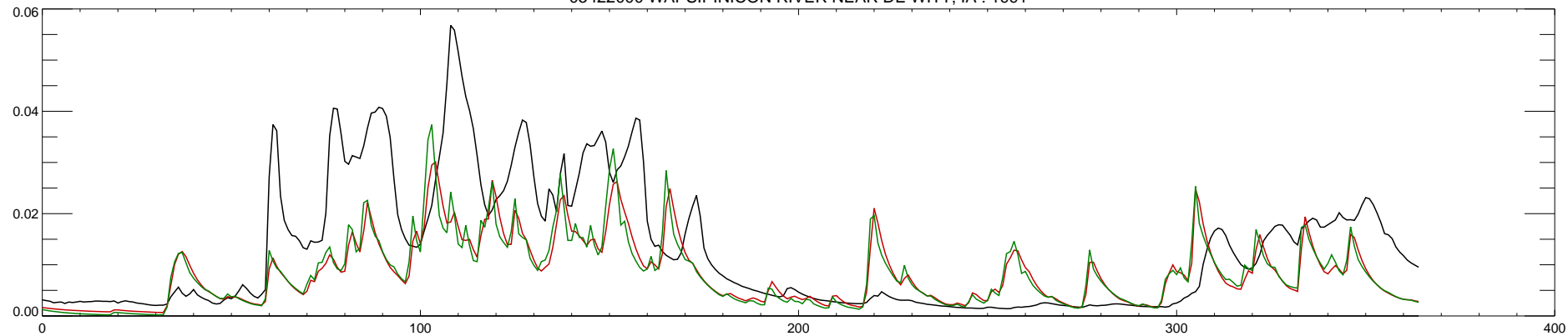
05422000 WAPSIPINICON RIVER NEAR DE WITT, IA : 1992
