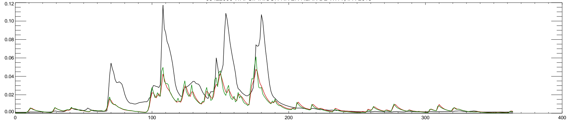
05422000 WAPSIPINICON RIVER NEAR DE WITT, IA : 2013
