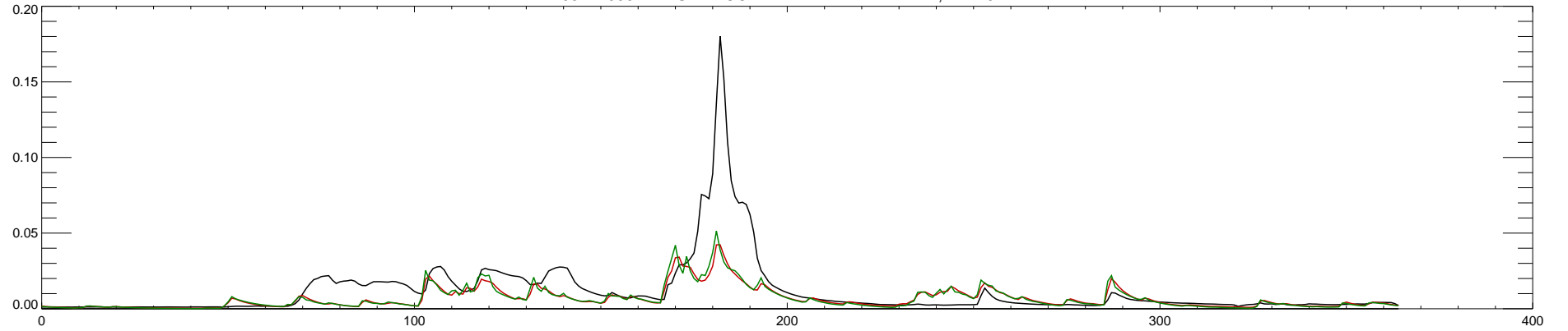
05422000 WAPSIPINICON RIVER NEAR DE WITT, IA : 2015
