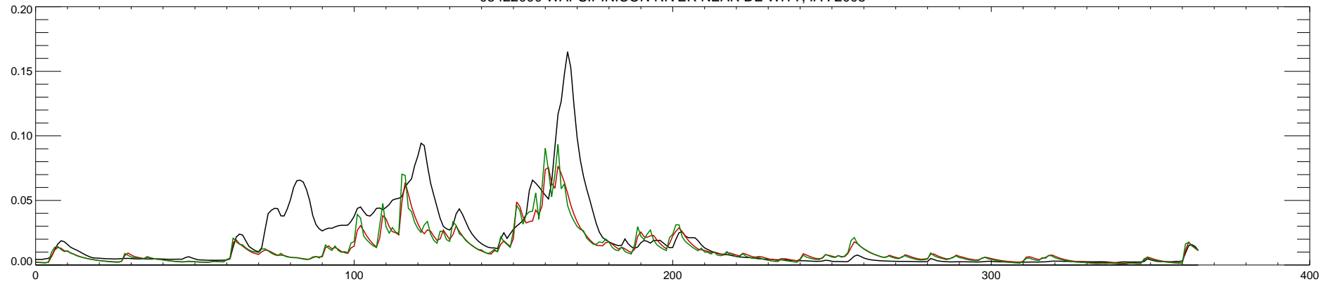
05422000 WAPSIPINICON RIVER NEAR DE WITT, IA : 2009
