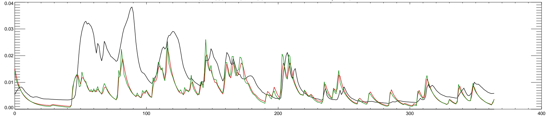
05422000 WAPSIPINICON RIVER NEAR DE WITT, IA : 2012
