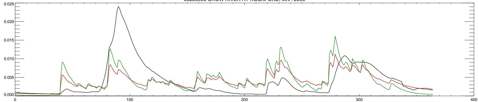
05280000 CROW RIVER AT ROCKFORD, MN : 2010
