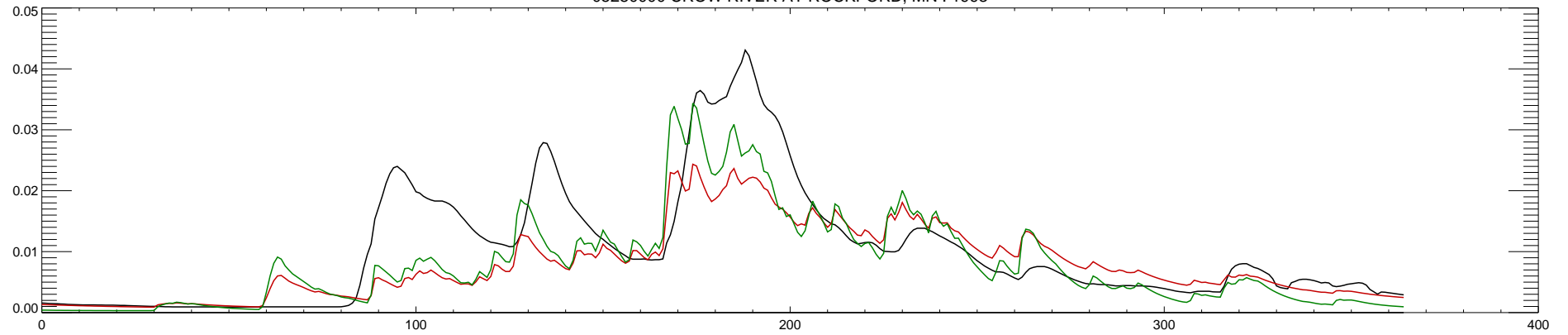
05280000 CROW RIVER AT ROCKFORD, MN : 1994
