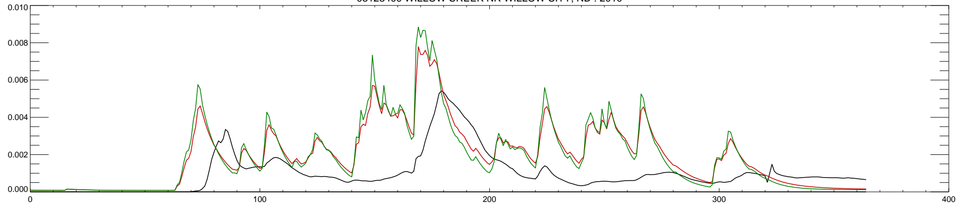
05123400 WILLOW CREEK NR WILLOW CITY, ND : 2010
