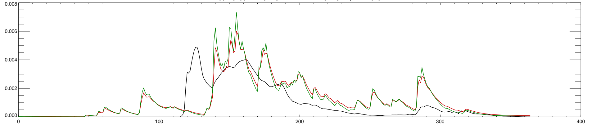
05123400 WILLOW CREEK NR WILLOW CITY, ND : 2013
