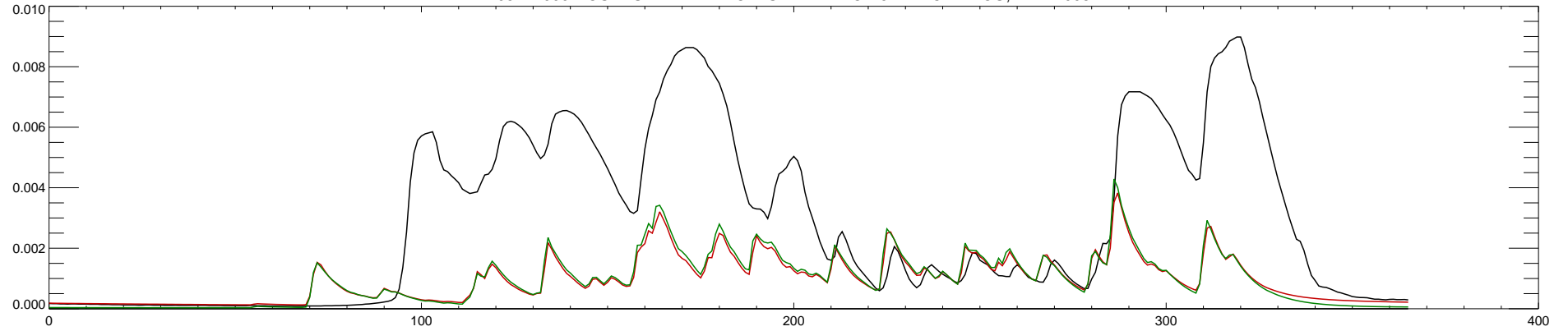
05112000 ROSEAU RIVER BELOW STATE DITCH 51 NR CARIBOU, MN : 2009
