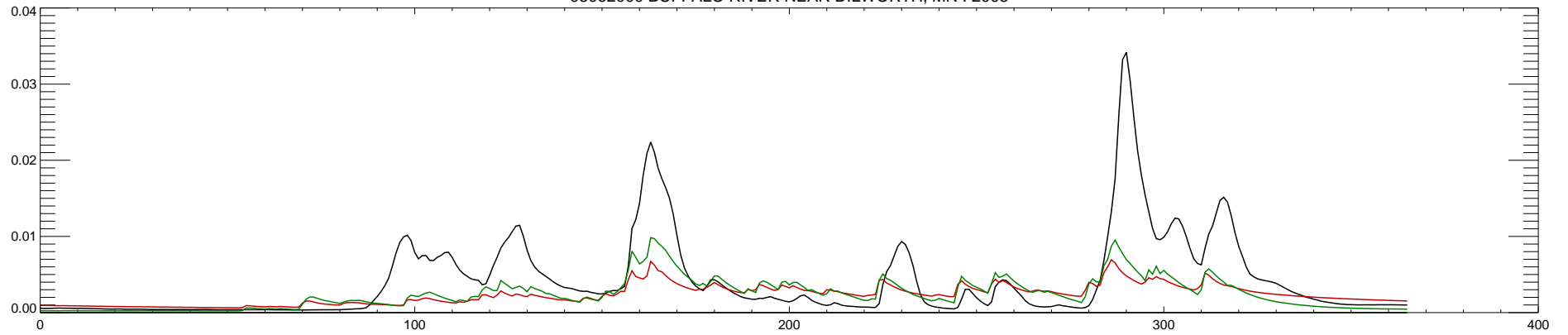
05062000 BUFFALO RIVER NEAR DILWORTH, MN : 2009
