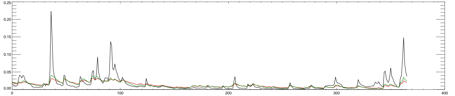
04223000 GENESEE RIVER AT PORTAGEVILLE NY : 2009
