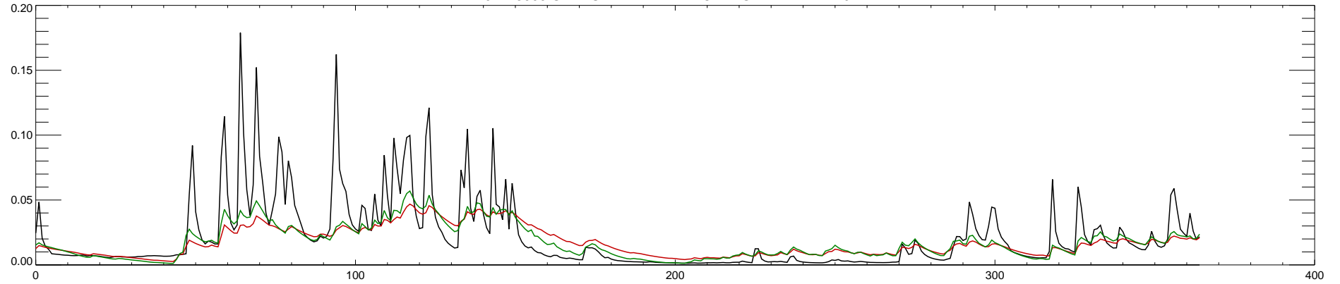
04223000 GENESEE RIVER AT PORTAGEVILLE NY : 2012
