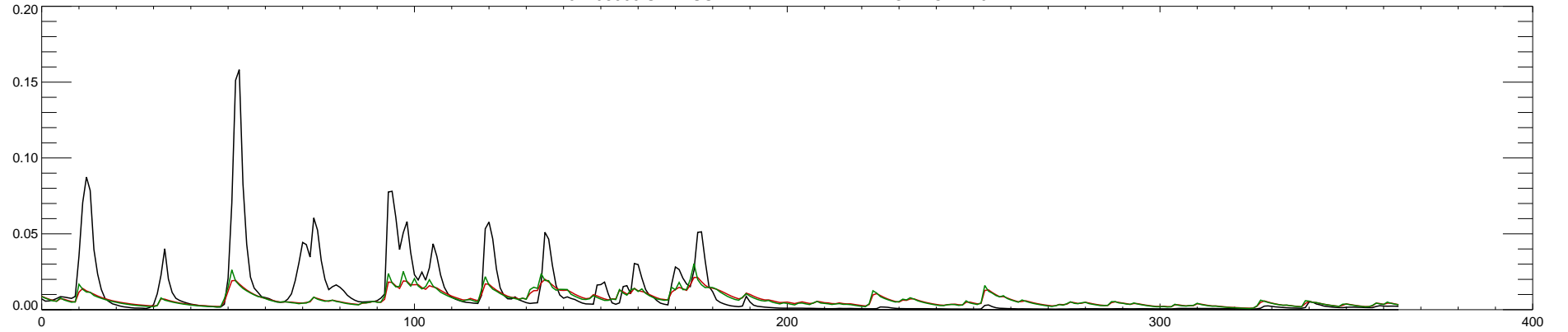
04198000 SANDUSKY RIVER NEAR FREMONT OH : 2015
