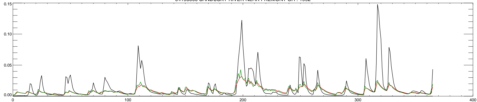
04198000 SANDUSKY RIVER NEAR FREMONT OH : 1992
