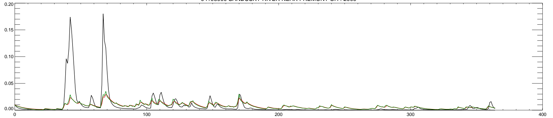
04198000 SANDUSKY RIVER NEAR FREMONT OH : 2010
