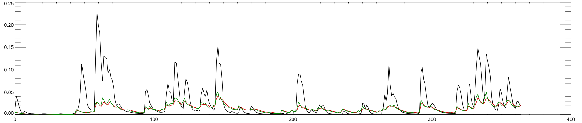
04198000 SANDUSKY RIVER NEAR FREMONT OH : 2012
