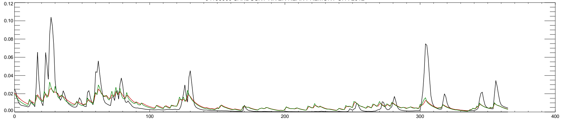
04198000 SANDUSKY RIVER NEAR FREMONT OH : 2013
