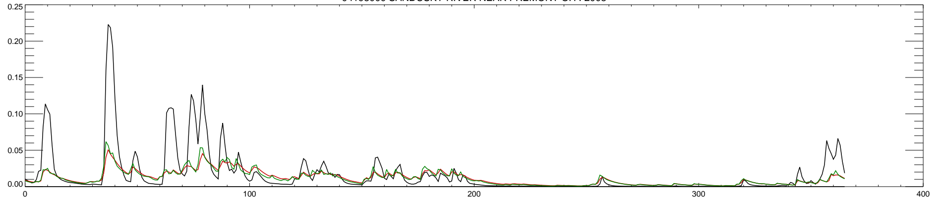
04198000 SANDUSKY RIVER NEAR FREMONT OH : 2009
