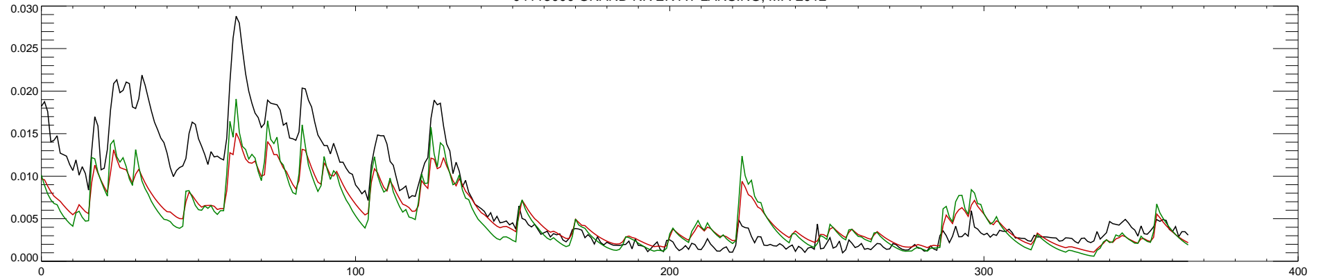
04113000 GRAND RIVER AT LANSING, MI : 2013
