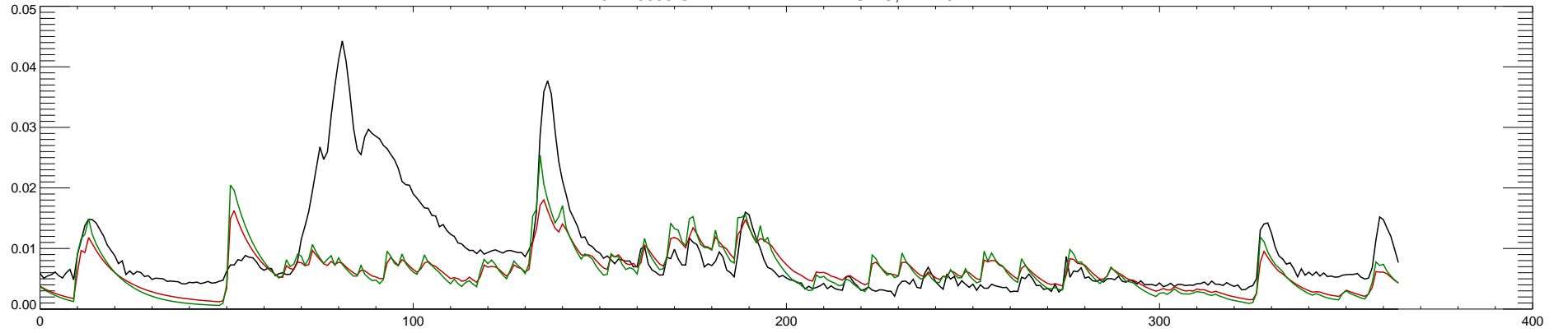
04113000 GRAND RIVER AT LANSING, MI : 2015
