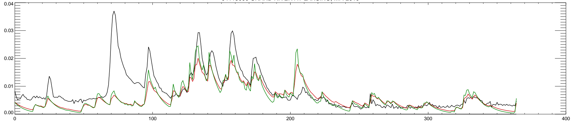
04113000 GRAND RIVER AT LANSING, MI : 2010
