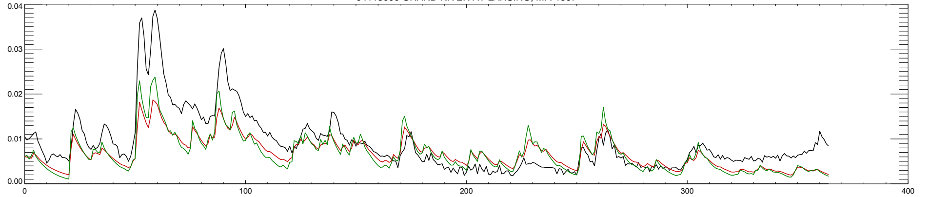
04113000 GRAND RIVER AT LANSING, MI : 1998
