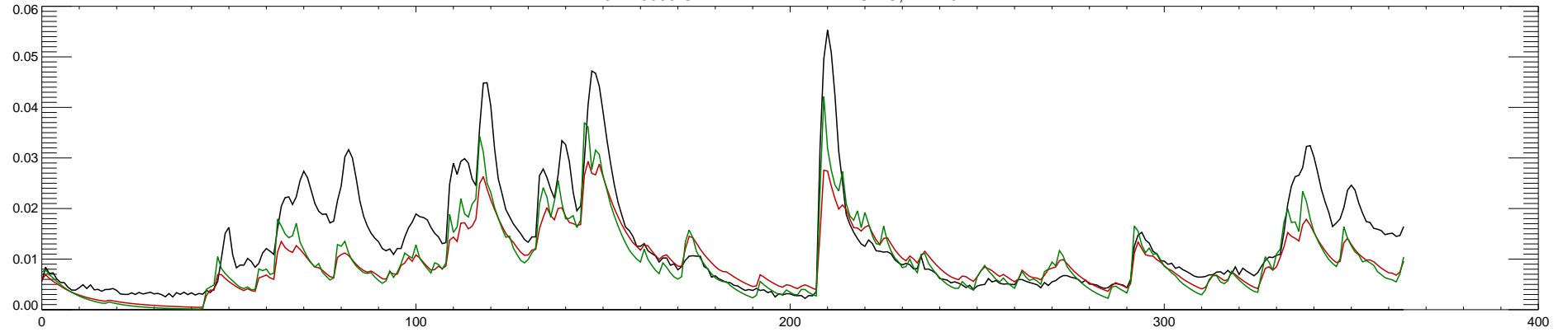
04113000 GRAND RIVER AT LANSING, MI : 2012
