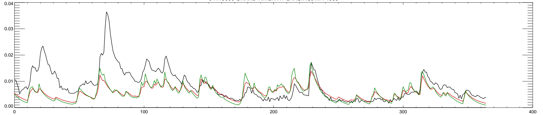
04113000 GRAND RIVER AT LANSING, MI : 1995
