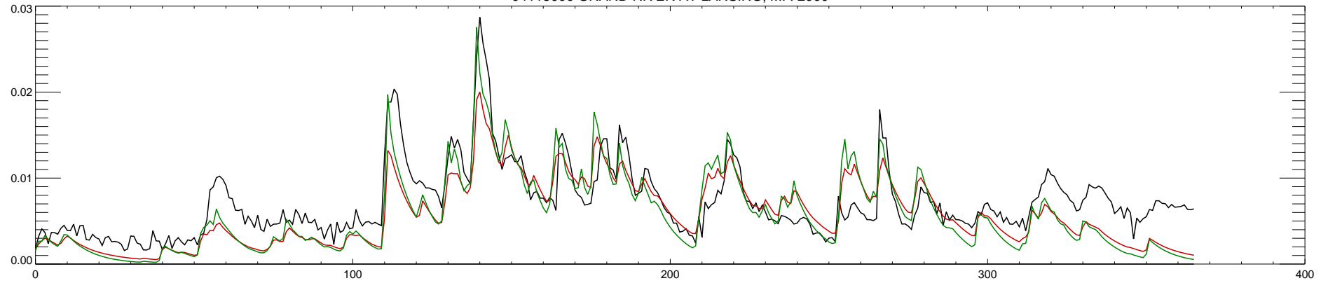
04113000 GRAND RIVER AT LANSING, MI : 2001
