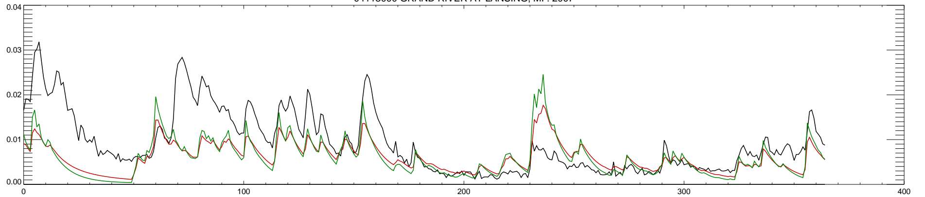
04113000 GRAND RIVER AT LANSING, MI : 2007
