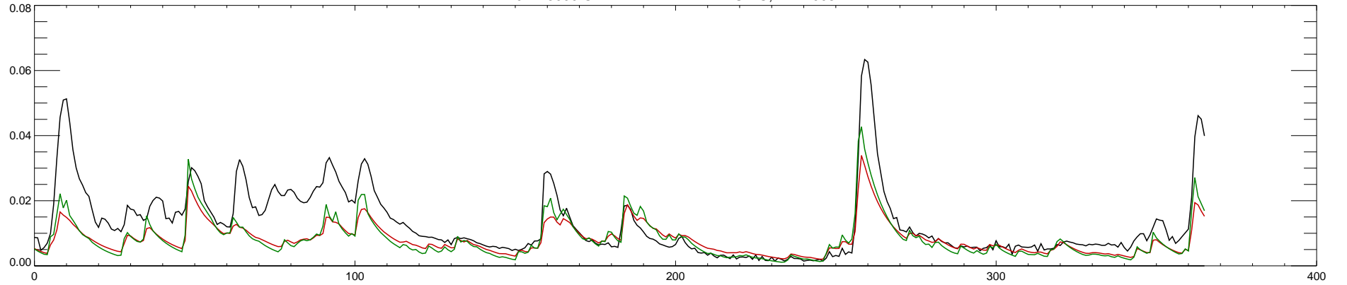
04113000 GRAND RIVER AT LANSING, MI : 2009
