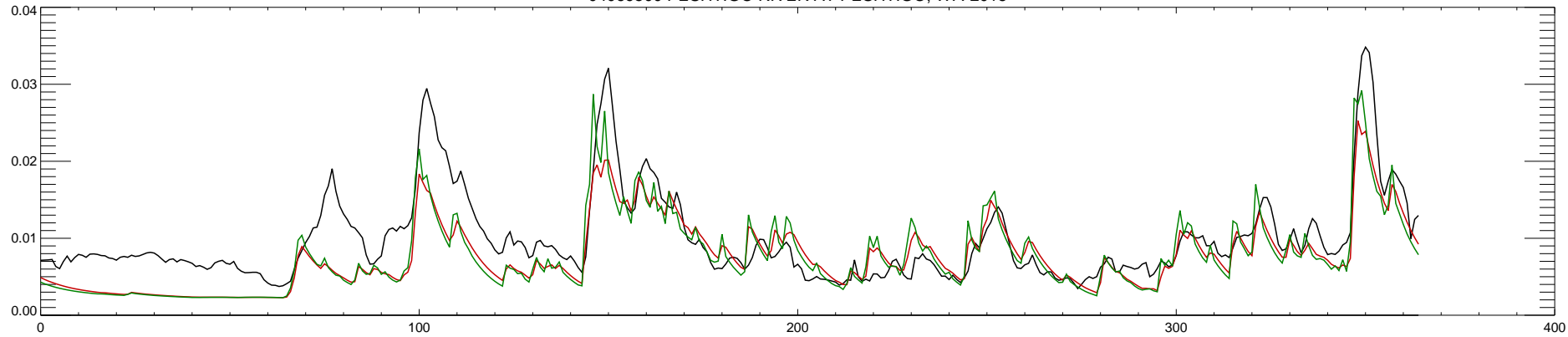
04069500 PESHTIGO RIVER AT PESHTIGO, WI : 2016
