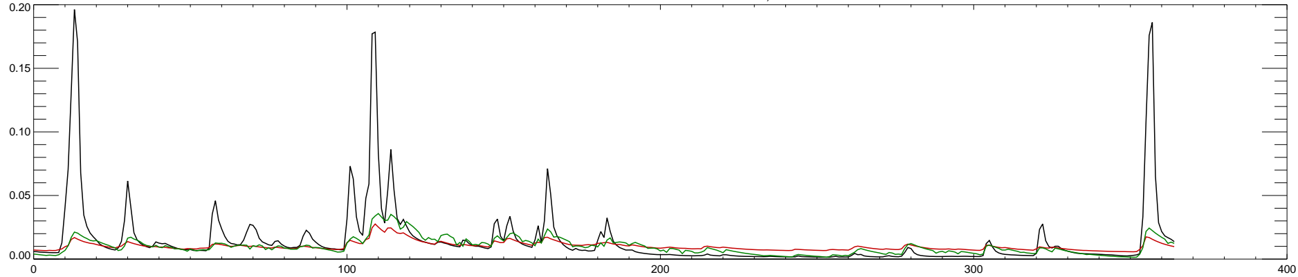
03349000 WHITE RIVER AT NOBLESVILLE, IN : 2013
