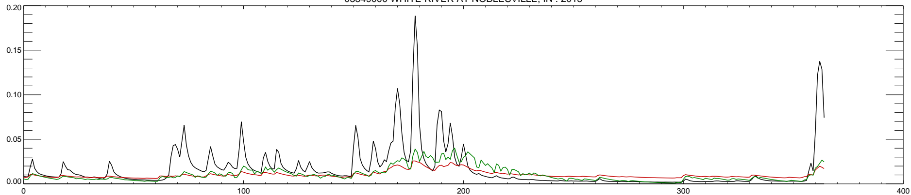
03349000 WHITE RIVER AT NOBLESVILLE, IN : 2016
