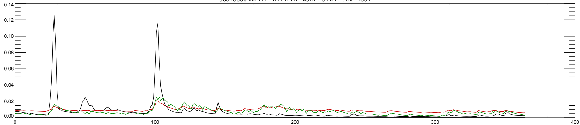
03349000 WHITE RIVER AT NOBLESVILLE, IN : 1995
