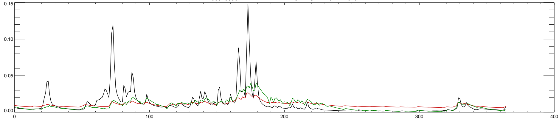
03349000 WHITE RIVER AT NOBLESVILLE, IN : 2010
