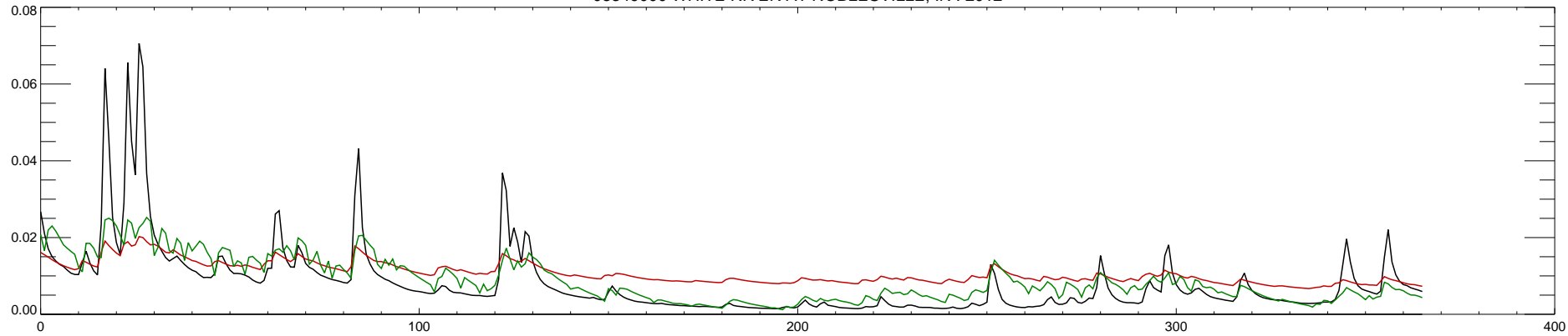
03349000 WHITE RIVER AT NOBLESVILLE, IN : 2013
