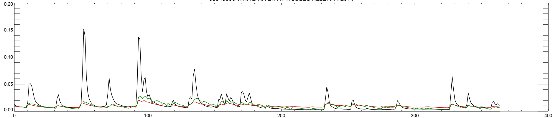
03349000 WHITE RIVER AT NOBLESVILLE, IN : 2015
