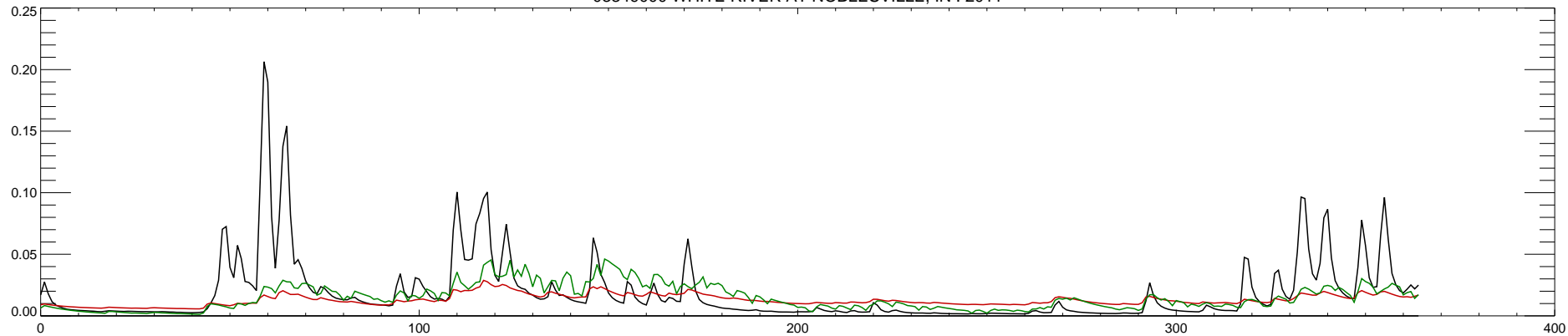
03349000 WHITE RIVER AT NOBLESVILLE, IN : 2012
