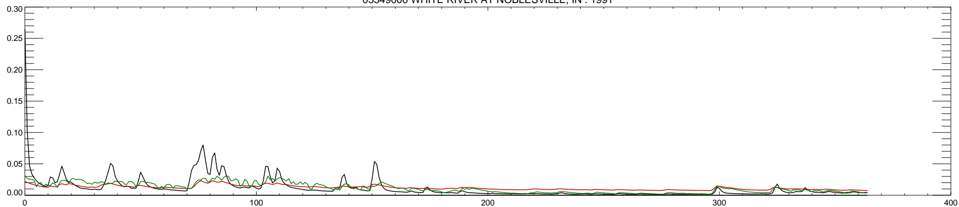
03349000 WHITE RIVER AT NOBLESVILLE, IN : 1992
