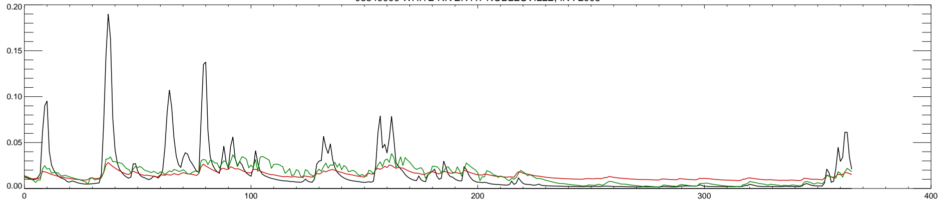
03349000 WHITE RIVER AT NOBLESVILLE, IN : 2009
