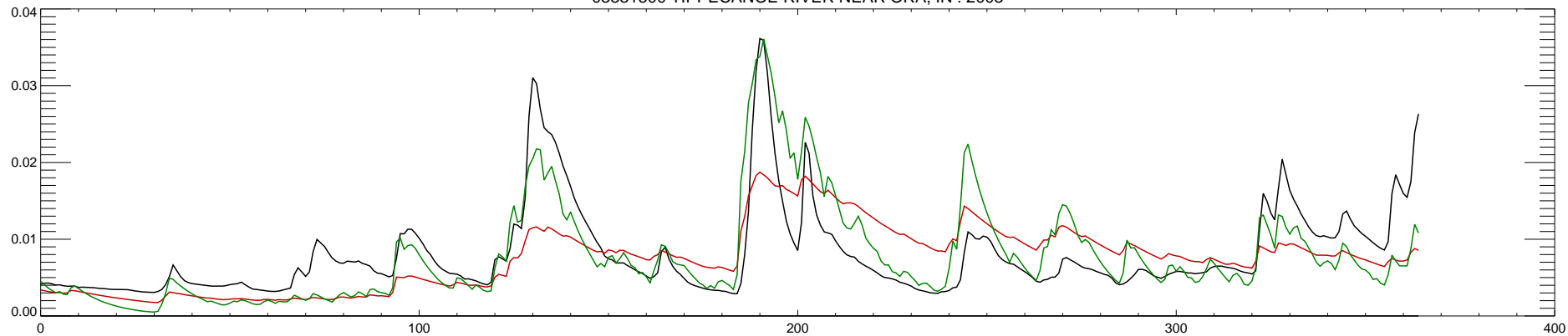
03331500 TIPPECANOE RIVER NEAR ORA, IN : 2004
